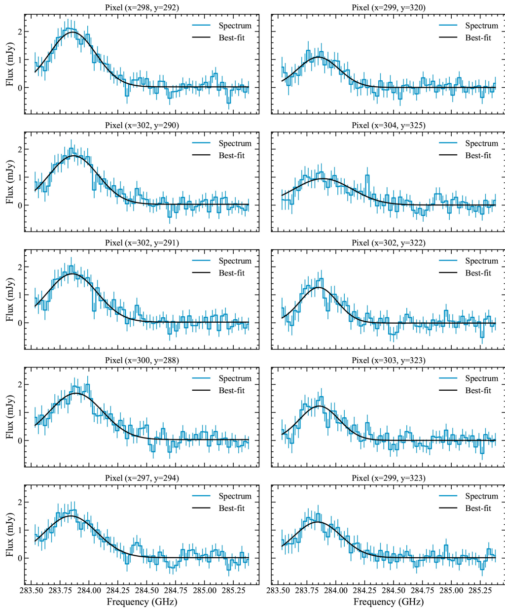
Figure 5. from Minghao Yue et al 2026 Astrophys. J. Lett. 1002 doi:10.3847/2041-8213/ae5e5b https://dx.doi.org/10.3847/2041-8213/ae5e5b © 2026. The Author(s). Published by the American Astronomical Society.
