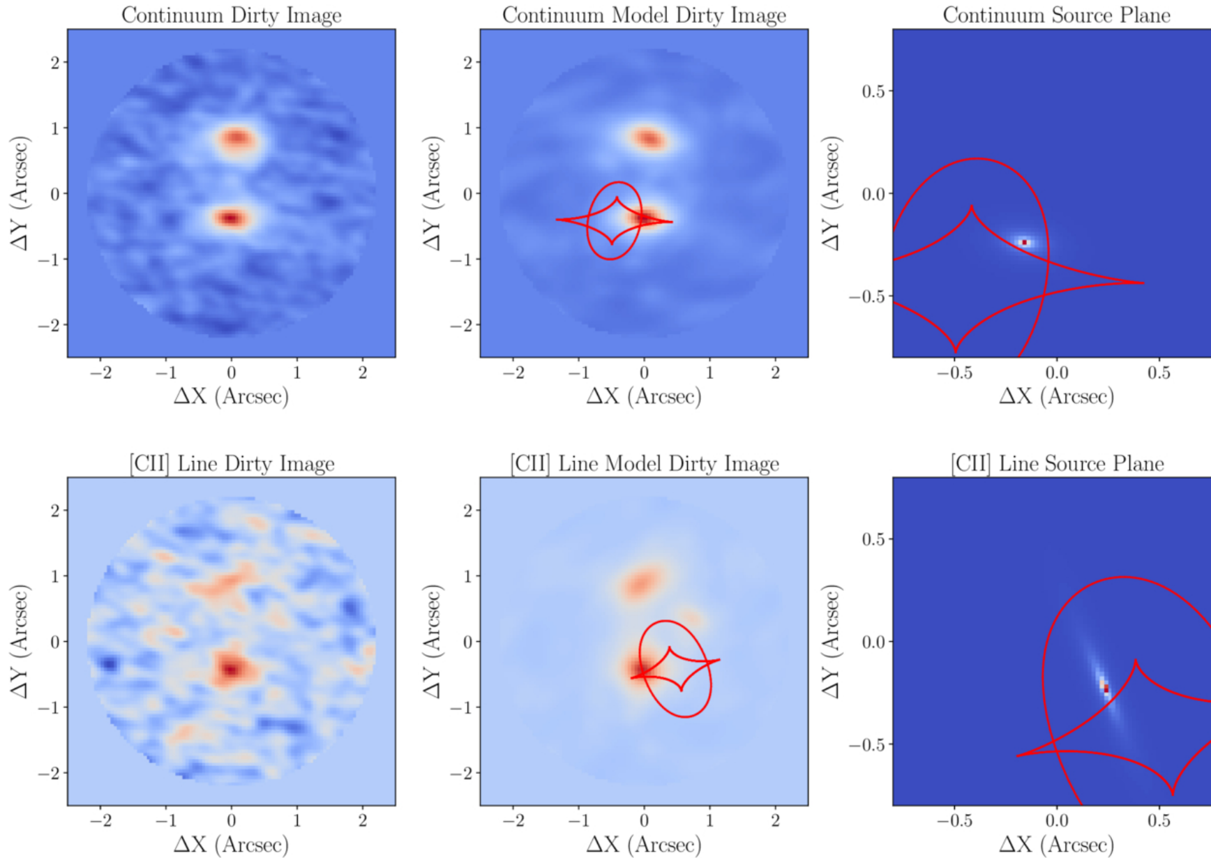
Figure 3. from Minghao Yue et al 2026 Astrophys. J. Lett. 1002 doi:10.3847/2041-8213/ae5e5b https://dx.doi.org/10.3847/2041-8213/ae5e5b © 2026. The Author(s). Published by the American Astronomical Society.
