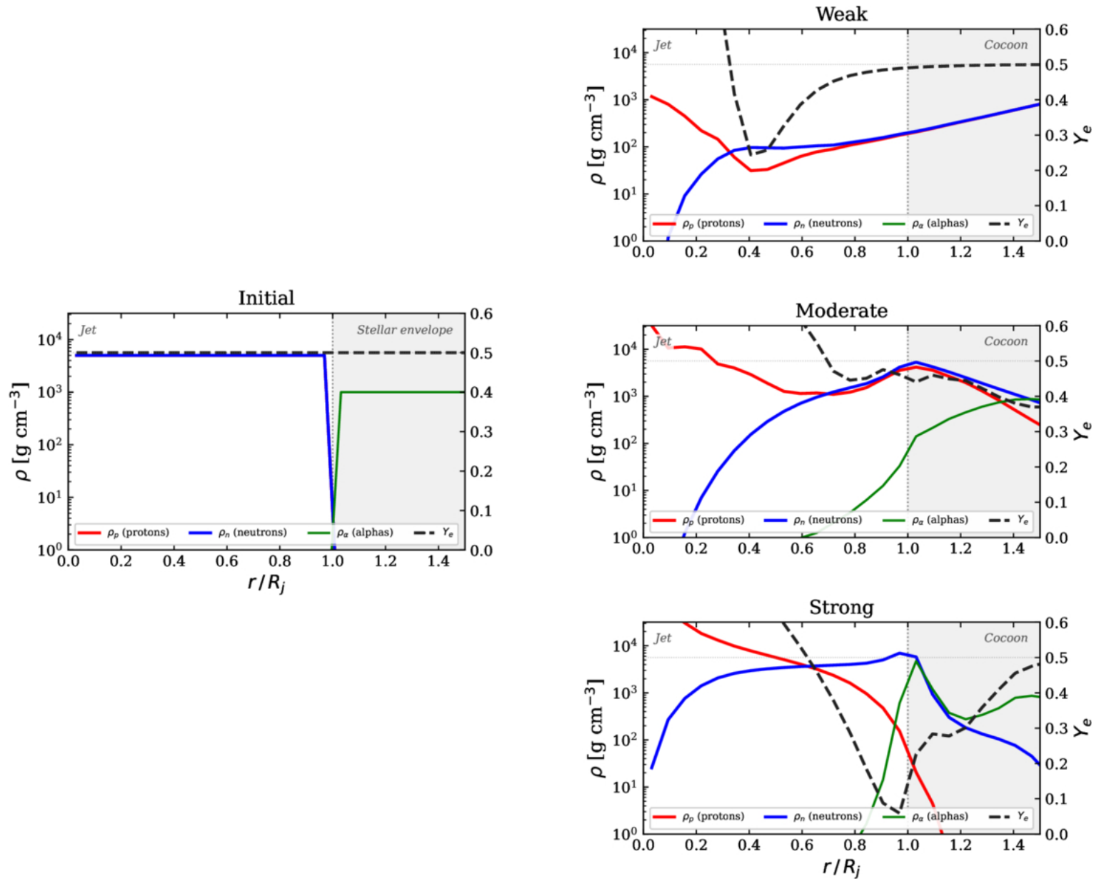
Figure 4. from Marko Risti et al 2026 Astrophys. J. Lett. 1002 doi:10.3847/2041-8213/ae5e53 https://dx.doi.org/10.3847/2041-8213/ae5e53 © 2026. The Author(s). Published by the American Astronomical Society.
