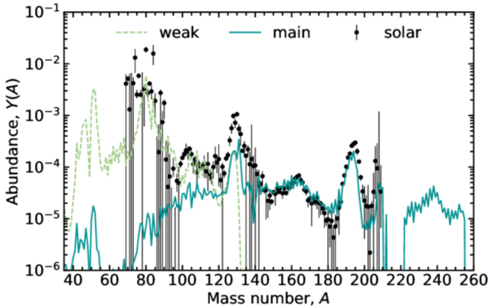
Figure 2. from Marko Risti et al 2026 Astrophys. J. Lett. 1002 doi:10.3847/2041-8213/ae5e53 https://dx.doi.org/10.3847/2041-8213/ae5e53 © 2026. The Author(s). Published by the American Astronomical Society.
