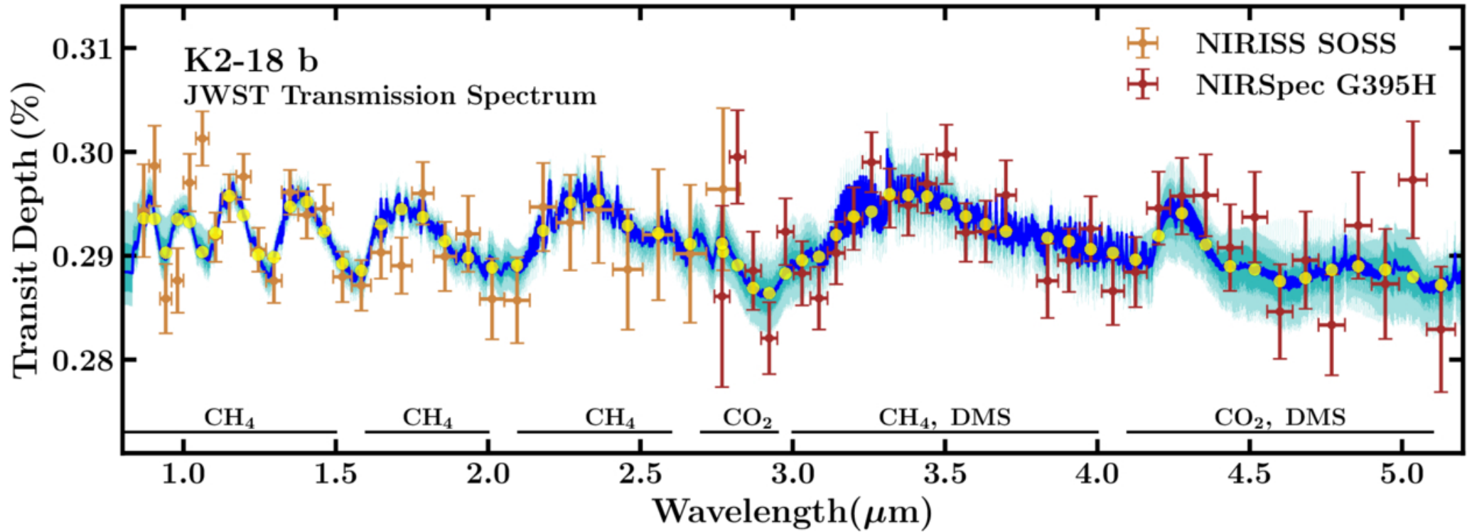
Figure 5. from Lorenzo Pica-Ciamarra et al 2026 Astrophys. J. Lett. 1002 doi:10.3847/2041-8213/ae5dcc https://dx.doi.org/10.3847/2041-8213/ae5dcc © 2026. The Author(s). Published by the American Astronomical Society.
