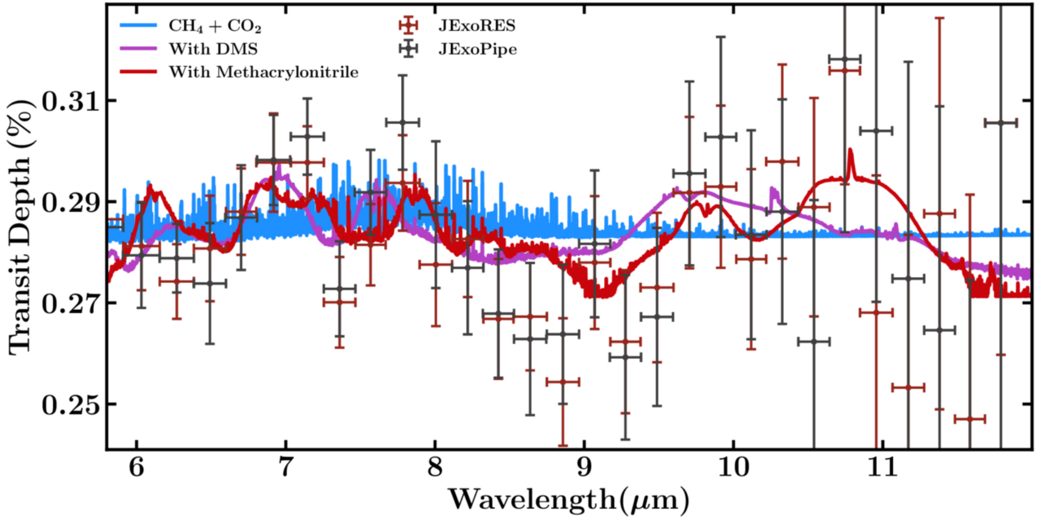
Figure 3. from Lorenzo Pica-Ciamarra et al 2026 Astrophys. J. Lett. 1002 doi:10.3847/2041-8213/ae5dcc https://dx.doi.org/10.3847/2041-8213/ae5dcc © 2026. The Author(s). Published by the American Astronomical Society.
