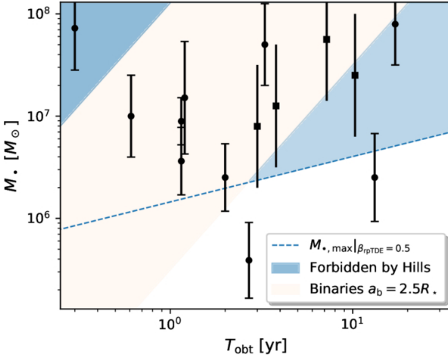
Figure 9. from Zhen Pan and Dong Lai 2026 Astrophys. J. Lett. 1002 doi:10.3847/2041-8213/ae5d44 https://dx.doi.org/10.3847/2041-8213/ae5d44 © 2026. The Author(s). Published by the American Astronomical Society.
