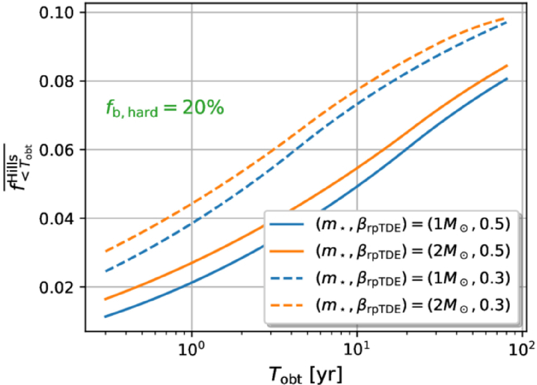
Figure 8. from Zhen Pan and Dong Lai 2026 Astrophys. J. Lett. 1002 doi:10.3847/2041-8213/ae5d44 https://dx.doi.org/10.3847/2041-8213/ae5d44 © 2026. The Author(s). Published by the American Astronomical Society.
