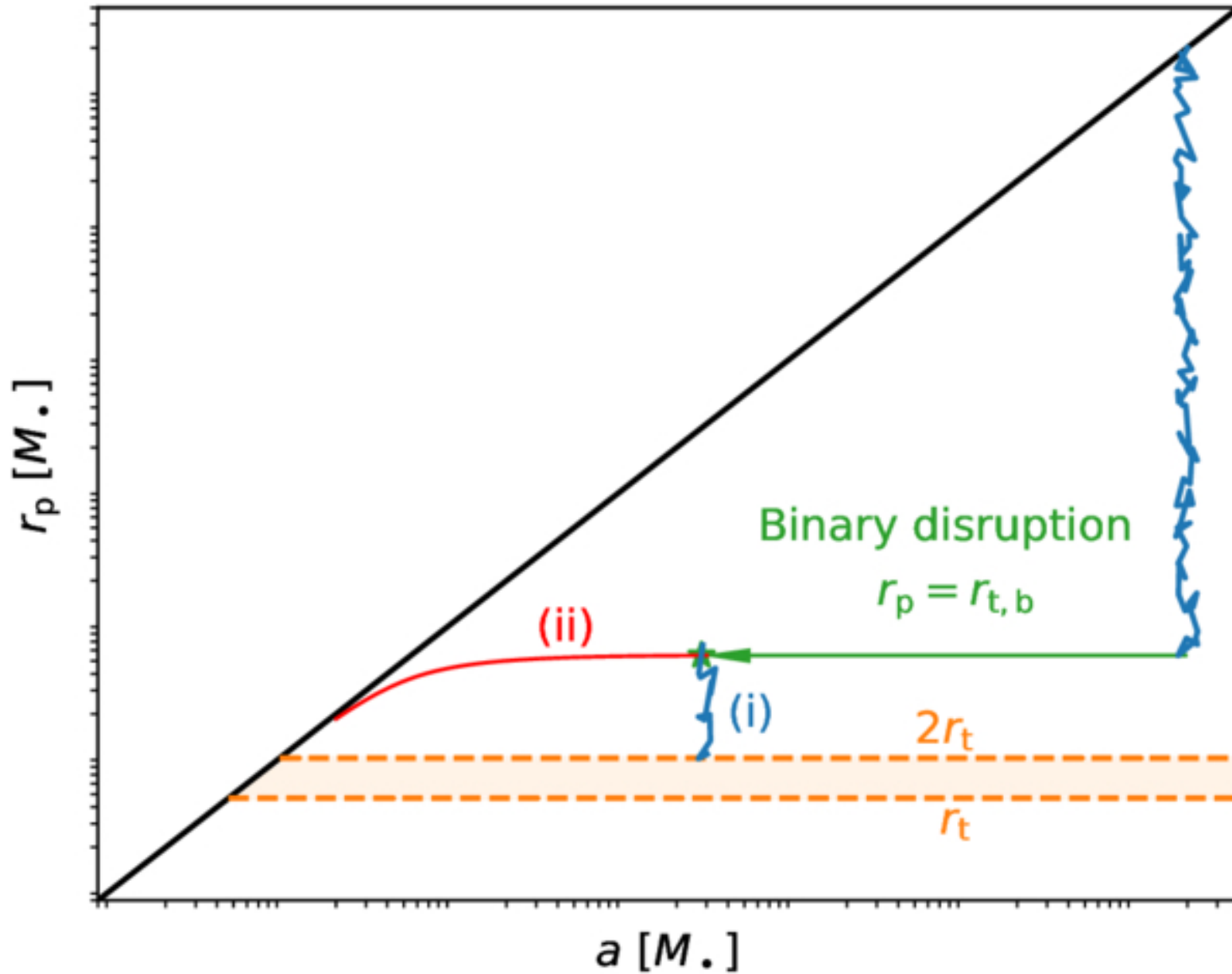
Figure 5. from Zhen Pan and Dong Lai 2026 Astrophys. J. Lett. 1002 doi:10.3847/2041-8213/ae5d44 https://dx.doi.org/10.3847/2041-8213/ae5d44 © 2026. The Author(s). Published by the American Astronomical Society.
