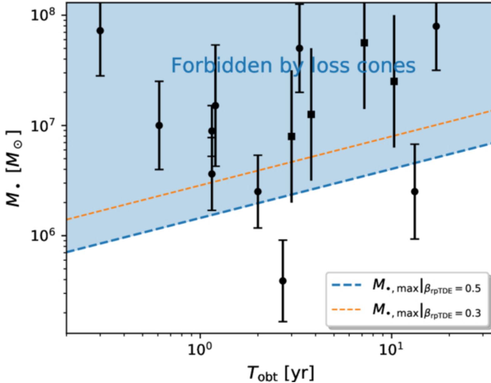
Figure 4. from Zhen Pan and Dong Lai 2026 Astrophys. J. Lett. 1002 doi:10.3847/2041-8213/ae5d44 https://dx.doi.org/10.3847/2041-8213/ae5d44 © 2026. The Author(s). Published by the American Astronomical Society.
