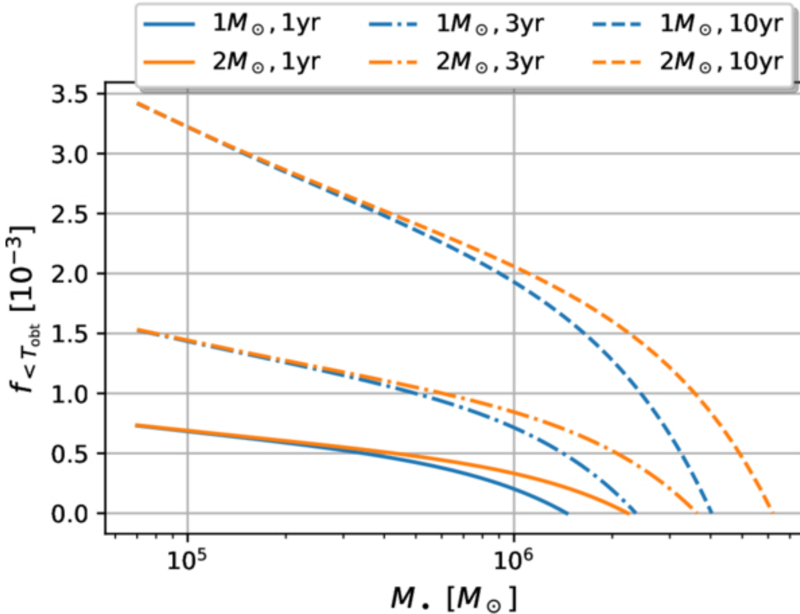
Figure 2. from Zhen Pan and Dong Lai 2026 Astrophys. J. Lett. 1002 doi:10.3847/2041-8213/ae5d44 https://dx.doi.org/10.3847/2041-8213/ae5d44 © 2026. The Author(s). Published by the American Astronomical Society.
