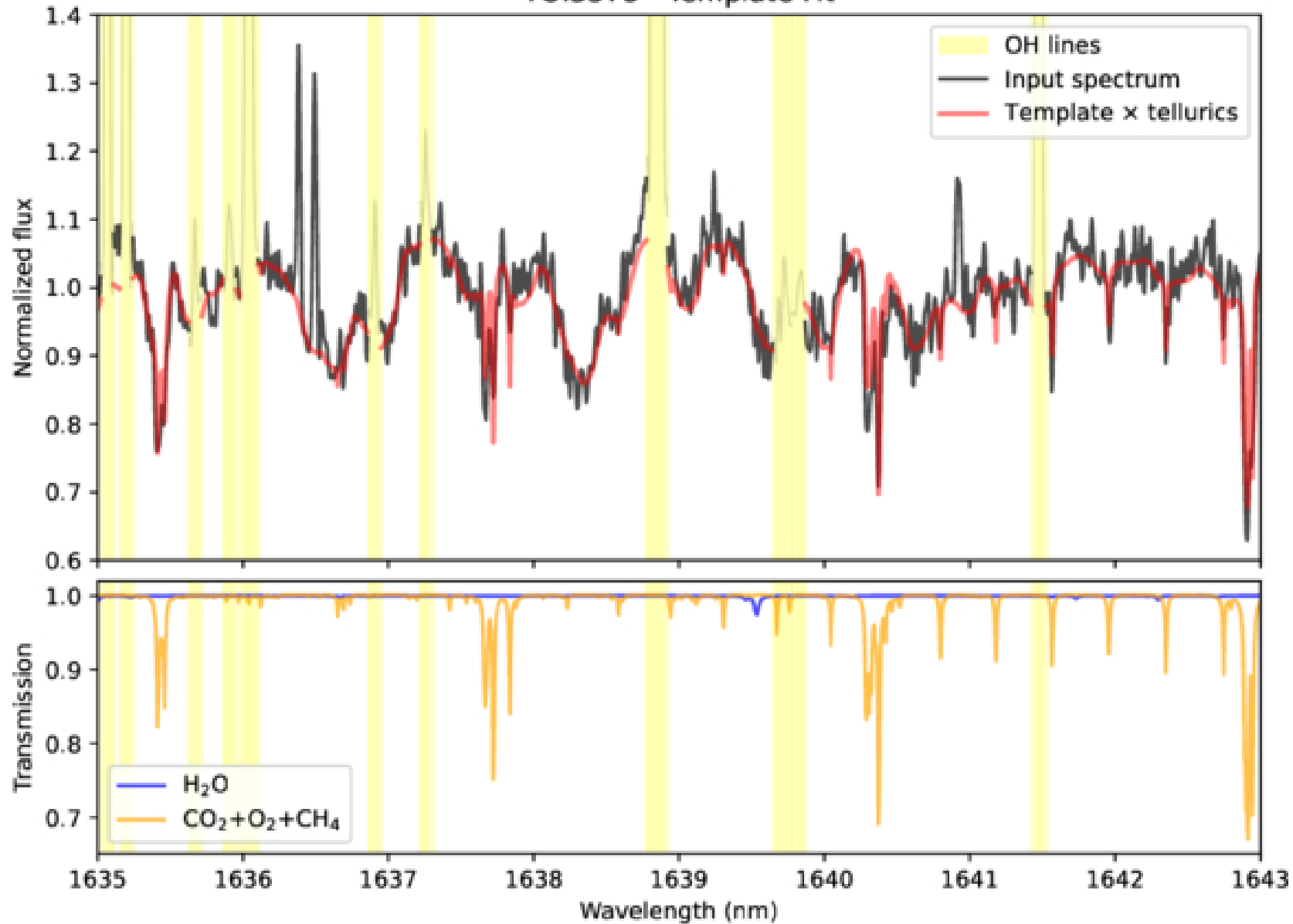
Figure A1. from Tianjun Gan et al 2026 Astrophys. J. Lett. 1002 doi:10.3847/2041-8213/ae5c95 https://dx.doi.org/10.3847/2041-8213/ae5c95 © 2026. The Author(s). Published by the American Astronomical Society.
