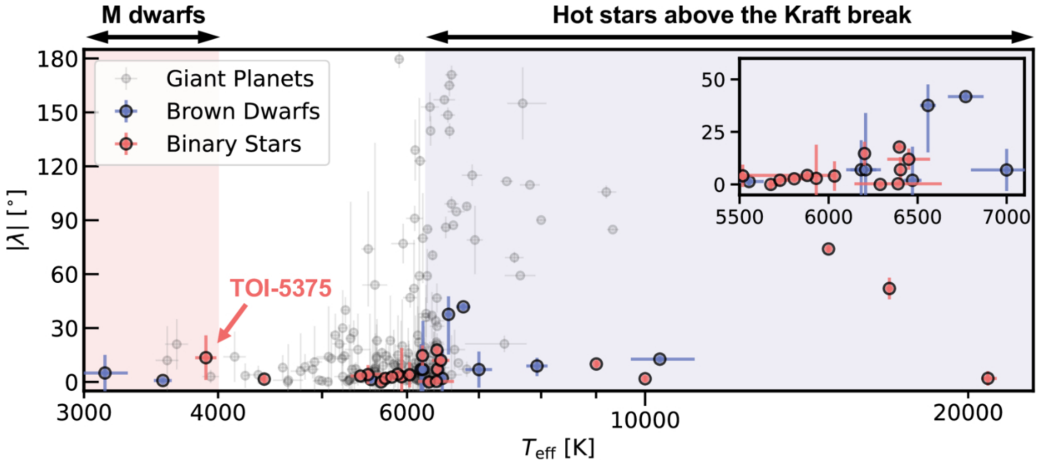
Figure 2. from Tianjun Gan et al 2026 Astrophys. J. Lett. 1002 doi:10.3847/2041-8213/ae5c95 https://dx.doi.org/10.3847/2041-8213/ae5c95 © 2026. The Author(s). Published by the American Astronomical Society.
