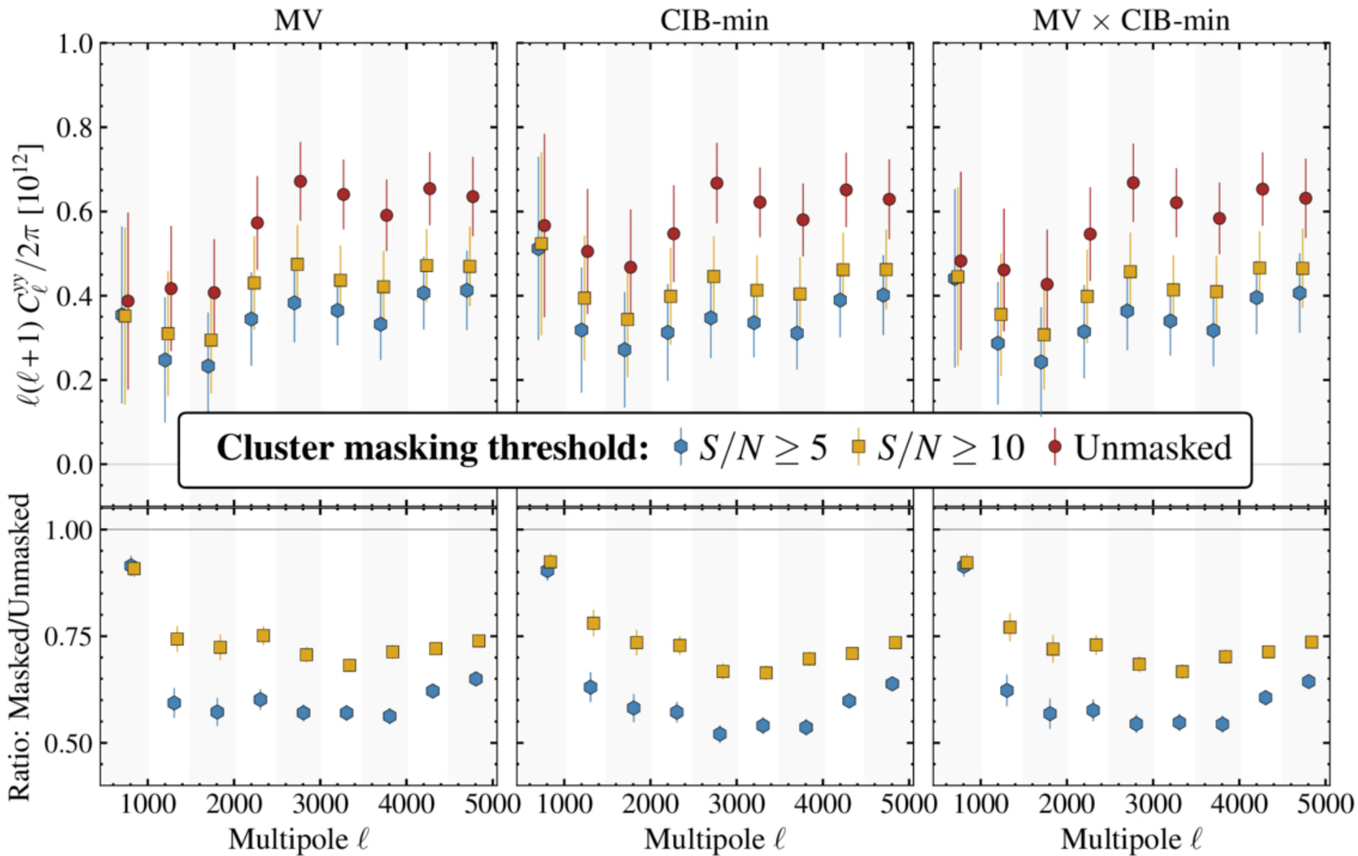
Figure 9. from S. Raghunathan et al 2026 Astrophys. J. Lett. 1002 doi:10.3847/2041-8213/ae5c07 https://dx.doi.org/10.3847/2041-8213/ae5c07 © 2026. The Author(s). Published by the American Astronomical Society.
