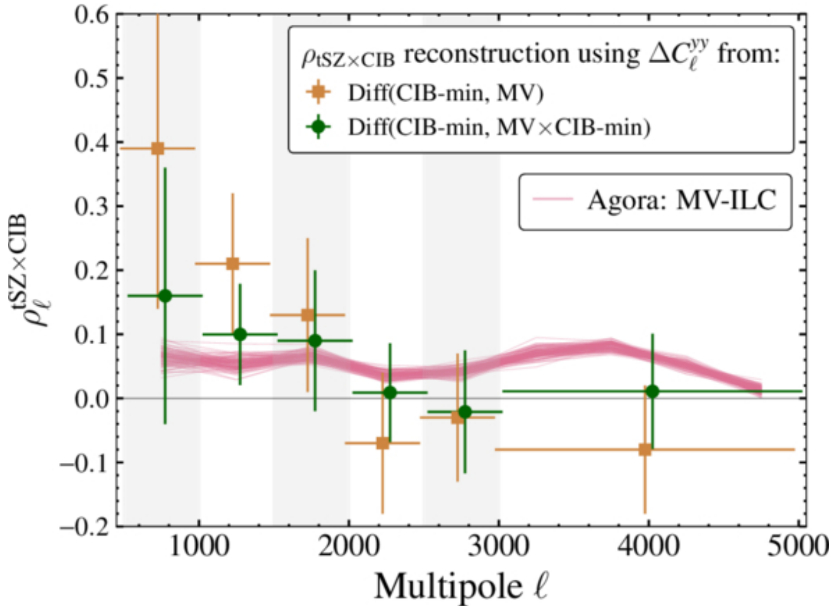
Figure 7. from S. Raghunathan et al 2026 Astrophys. J. Lett. 1002 doi:10.3847/2041-8213/ae5c07 https://dx.doi.org/10.3847/2041-8213/ae5c07 © 2026. The Author(s). Published by the American Astronomical Society.
