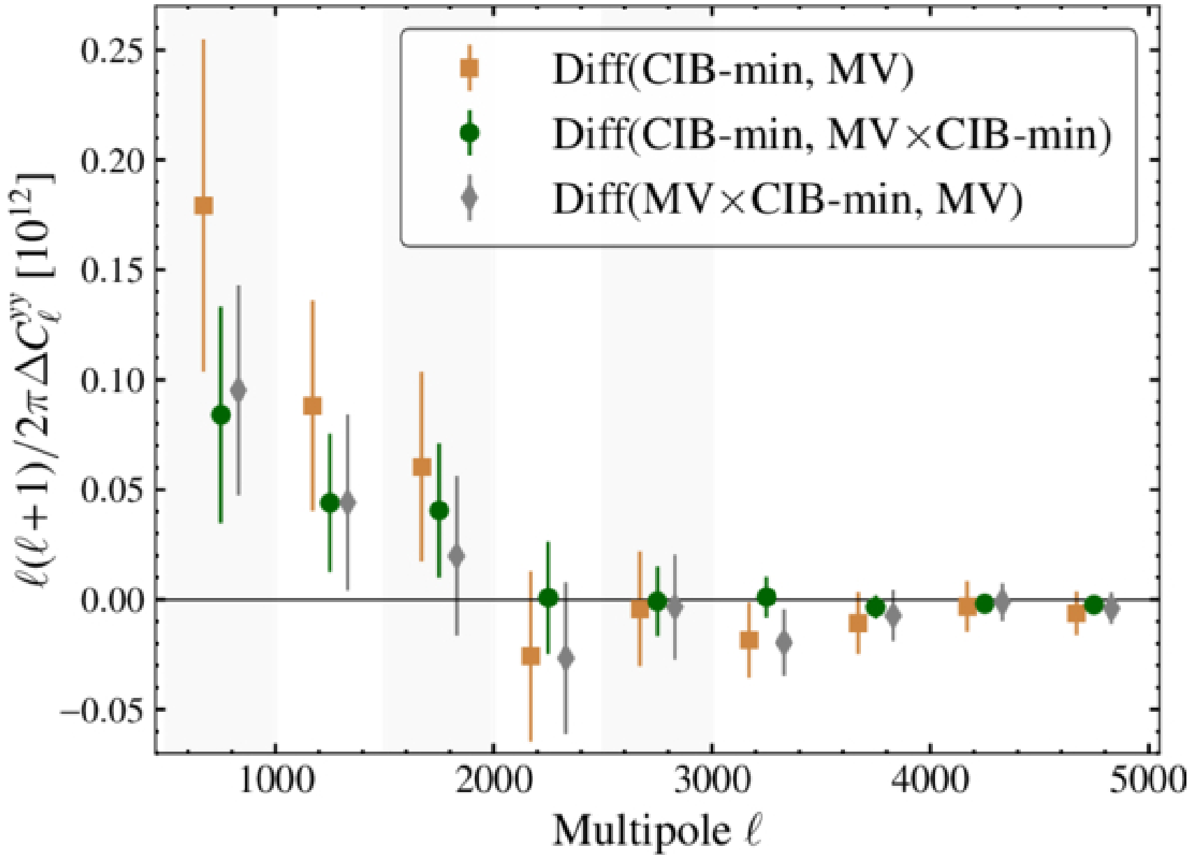
Figure 6. from S. Raghunathan et al 2026 Astrophys. J. Lett. 1002 doi:10.3847/2041-8213/ae5c07 https://dx.doi.org/10.3847/2041-8213/ae5c07 © 2026. The Author(s). Published by the American Astronomical Society.
