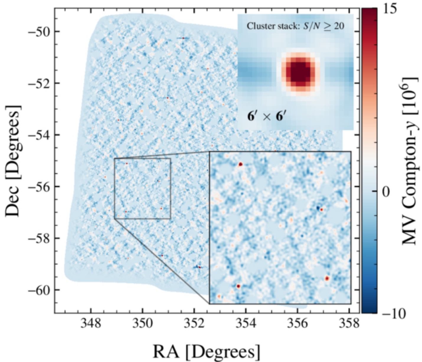
Figure 2. from S. Raghunathan et al 2026 Astrophys. J. Lett. 1002 doi:10.3847/2041-8213/ae5c07 https://dx.doi.org/10.3847/2041-8213/ae5c07 © 2026. The Author(s). Published by the American Astronomical Society.
