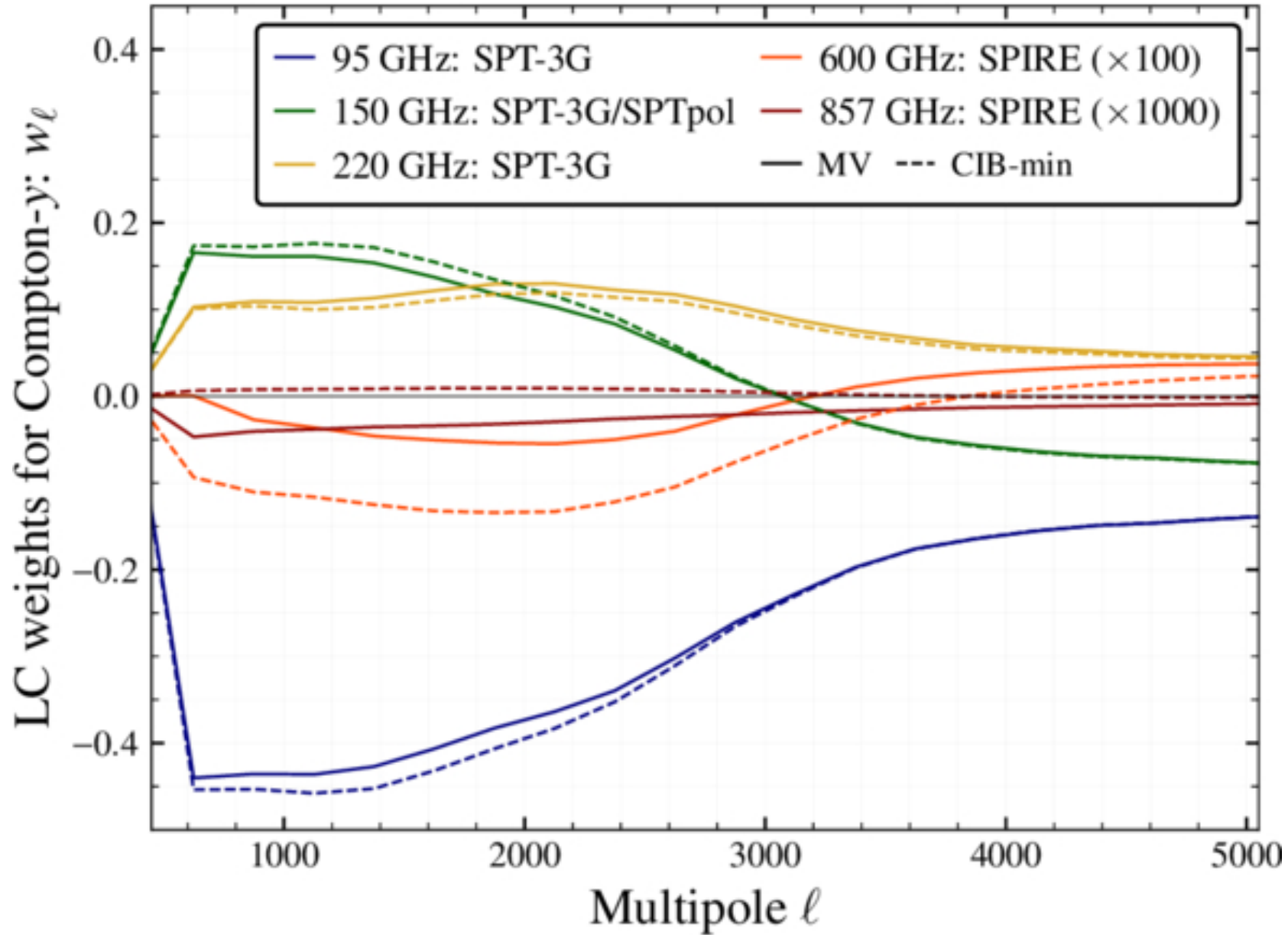
Figure 1. from S. Raghunathan et al 2026 Astrophys. J. Lett. 1002 doi:10.3847/2041-8213/ae5c07 https://dx.doi.org/10.3847/2041-8213/ae5c07 © 2026. The Author(s). Published by the American Astronomical Society.
