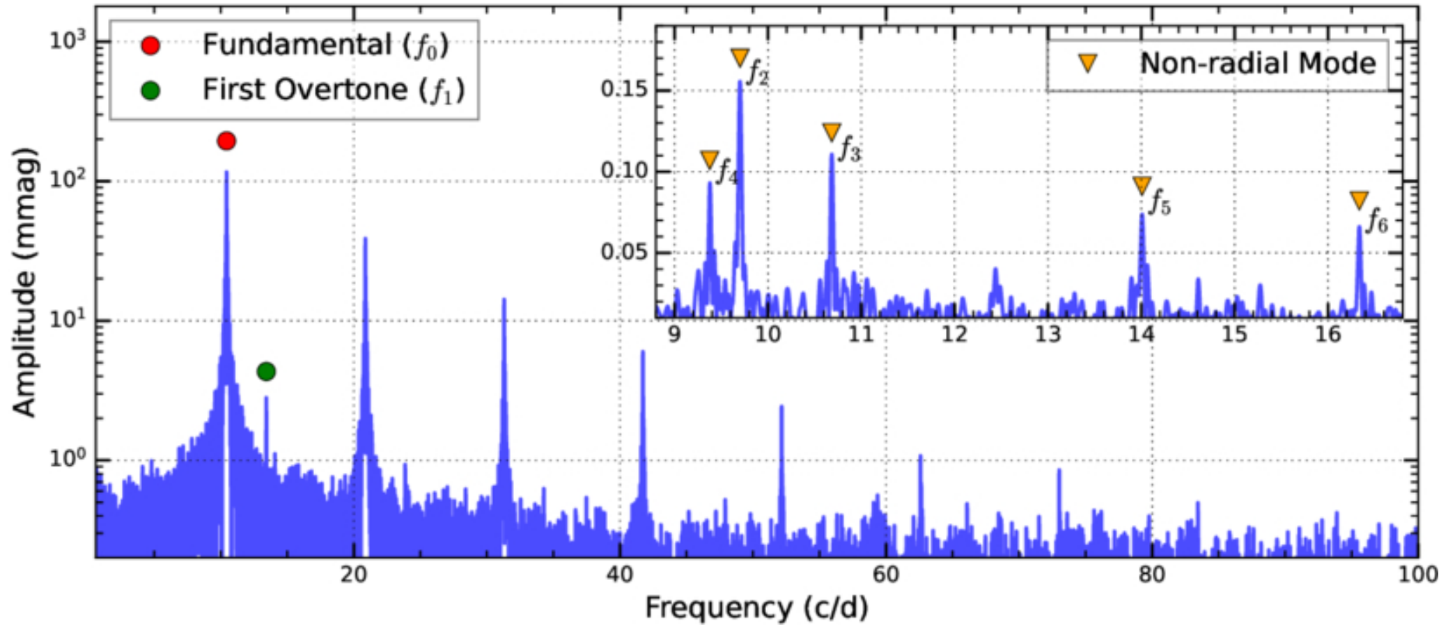
Figure 5. from Jia-Shu Niu et al 2026 Astrophys. J. Lett. 1001 doi:10.3847/2041-8213/ae5be3 https://dx.doi.org/10.3847/2041-8213/ae5be3 © 2026. The Author(s). Published by the American Astronomical Society.
