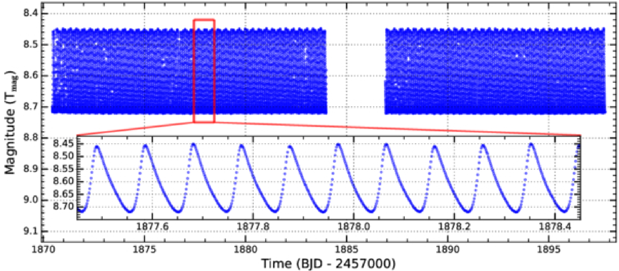
Figure 4. from Jia-Shu Niu et al 2026 Astrophys. J. Lett. 1001 doi:10.3847/2041-8213/ae5be3 https://dx.doi.org/10.3847/2041-8213/ae5be3 © 2026. The Author(s). Published by the American Astronomical Society.
