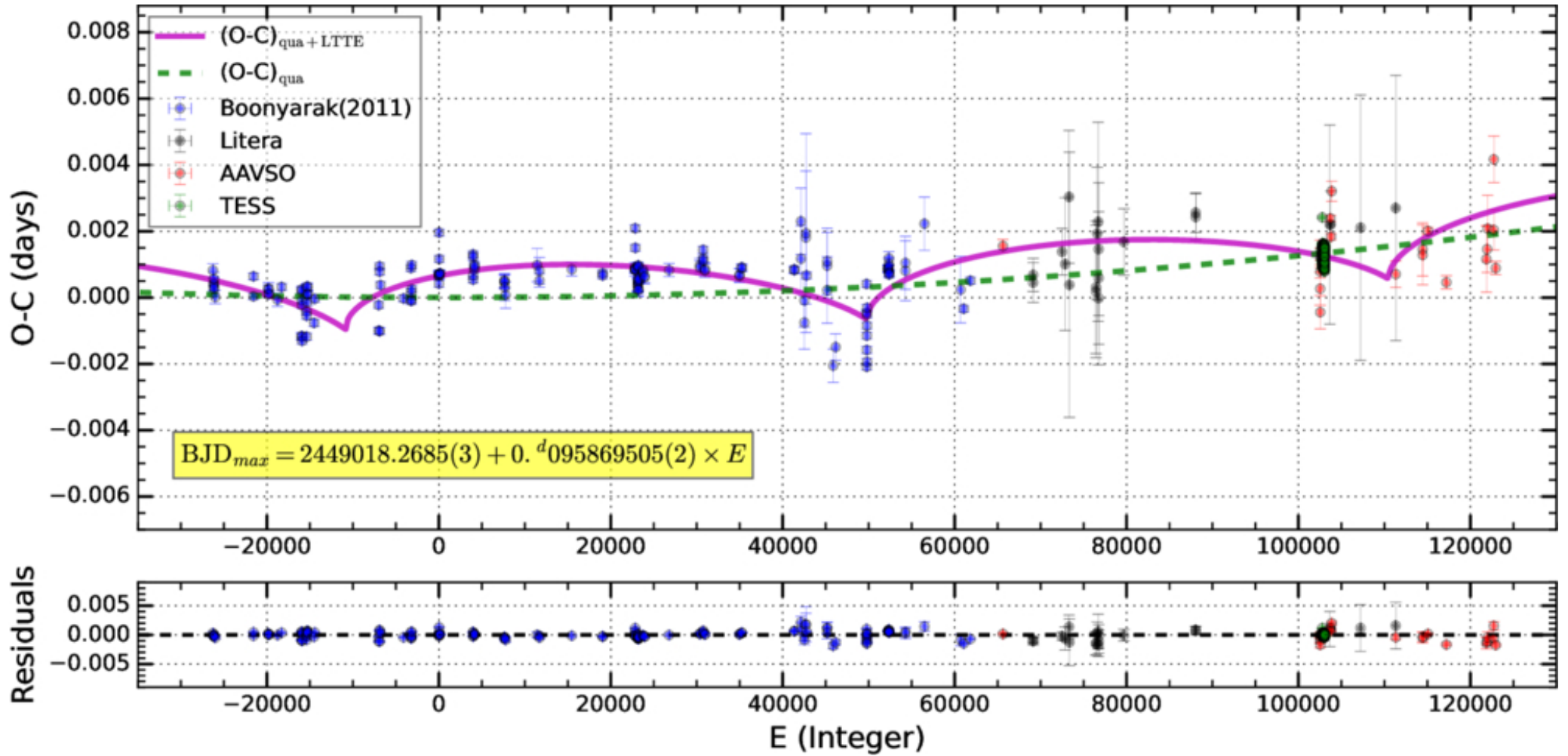
Figure 1. from Jia-Shu Niu et al 2026 Astrophys. J. Lett. 1001 doi:10.3847/2041-8213/ae5be3 https://dx.doi.org/10.3847/2041-8213/ae5be3 © 2026. The Author(s). Published by the American Astronomical Society.
