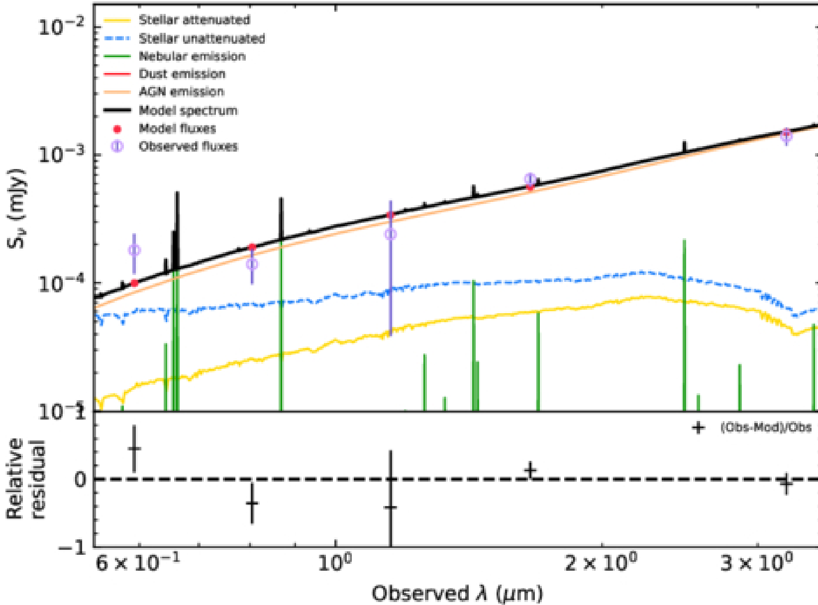
Figure A3. from Michael McDonald et al 2026 Astrophys. J. Lett. 1002 doi:10.3847/2041-8213/ae5bbe https://dx.doi.org/10.3847/2041-8213/ae5bbe © 2026. The Author(s). Published by the American Astronomical Society.
