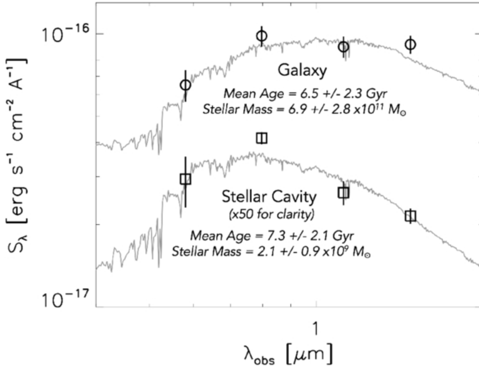
Figure A2. from Michael McDonald et al 2026 Astrophys. J. Lett. 1002 doi:10.3847/2041-8213/ae5bbe https://dx.doi.org/10.3847/2041-8213/ae5bbe © 2026. The Author(s). Published by the American Astronomical Society.
