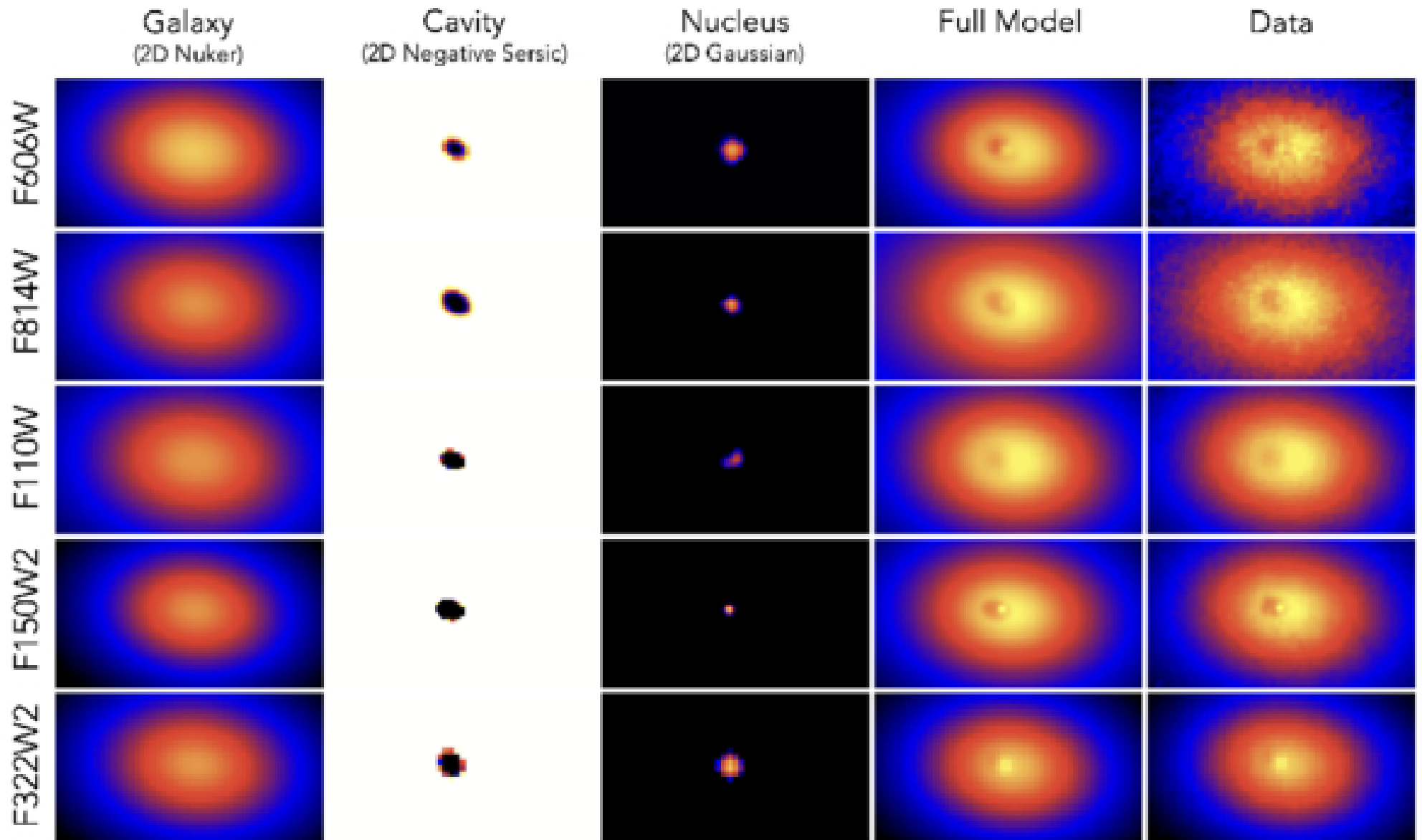
Figure A1. from Michael McDonald et al 2026 Astrophys. J. Lett. 1002 doi:10.3847/2041-8213/ae5bbe https://dx.doi.org/10.3847/2041-8213/ae5bbe © 2026. The Author(s). Published by the American Astronomical Society.
