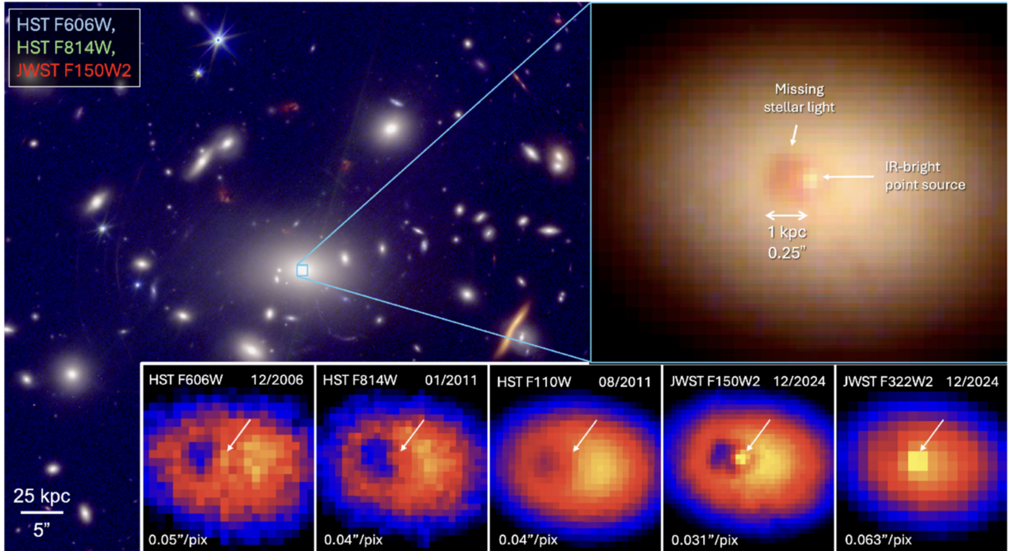
Figure 1. from Michael McDonald et al 2026 Astrophys. J. Lett. 1002 doi:10.3847/2041-8213/ae5bbe https://dx.doi.org/10.3847/2041-8213/ae5bbe © 2026. The Author(s). Published by the American Astronomical Society.
