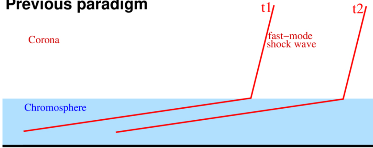
Figure 4. from C. H. Zhai et al 2026 Astrophys. J. Lett. 1001 doi:10.3847/2041-8213/ae5b9c https://dx.doi.org/10.3847/2041-8213/ae5b9c © 2026. The Author(s). Published by the American Astronomical Society.
