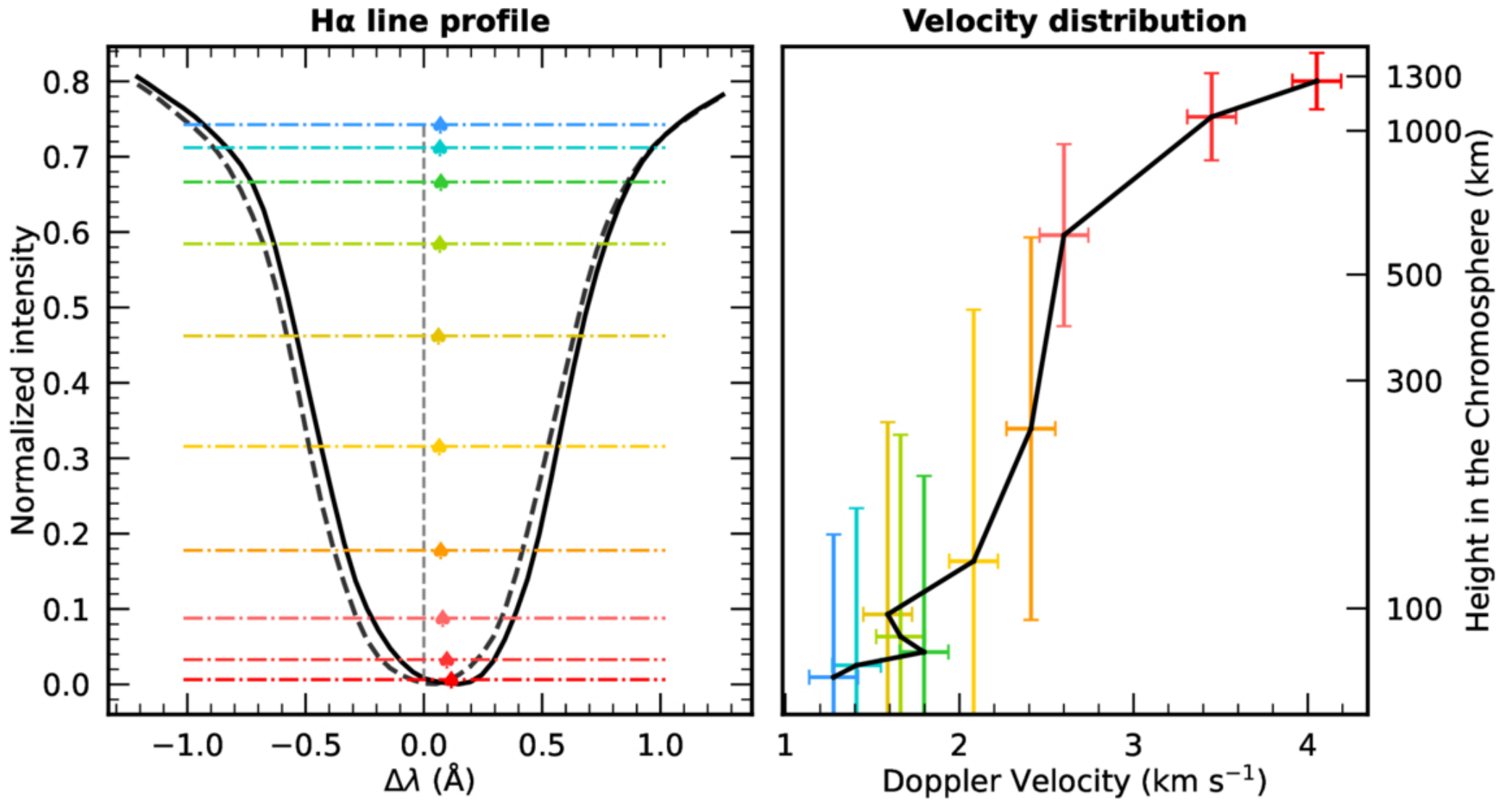
Figure 3. from C. H. Zhai et al 2026 Astrophys. J. Lett. 1001 doi:10.3847/2041-8213/ae5b9c https://dx.doi.org/10.3847/2041-8213/ae5b9c © 2026. The Author(s). Published by the American Astronomical Society.
