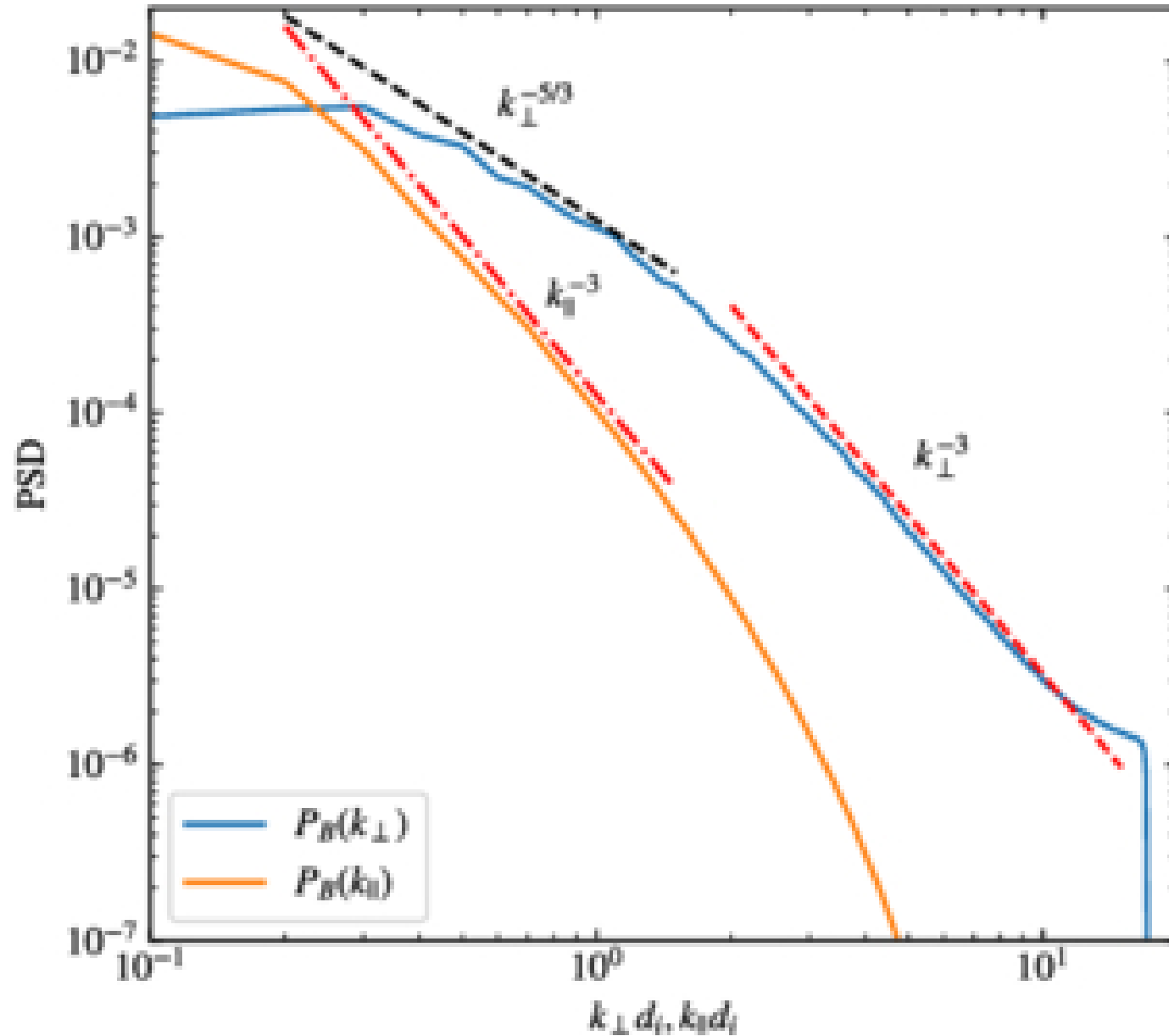
Figure 5. from Simone Benella et al 2026 Astrophys. J. Lett. 1001 doi:10.3847/2041-8213/ae5b81 https://dx.doi.org/10.3847/2041-8213/ae5b81 © 2026. The Author(s). Published by the American Astronomical Society.
