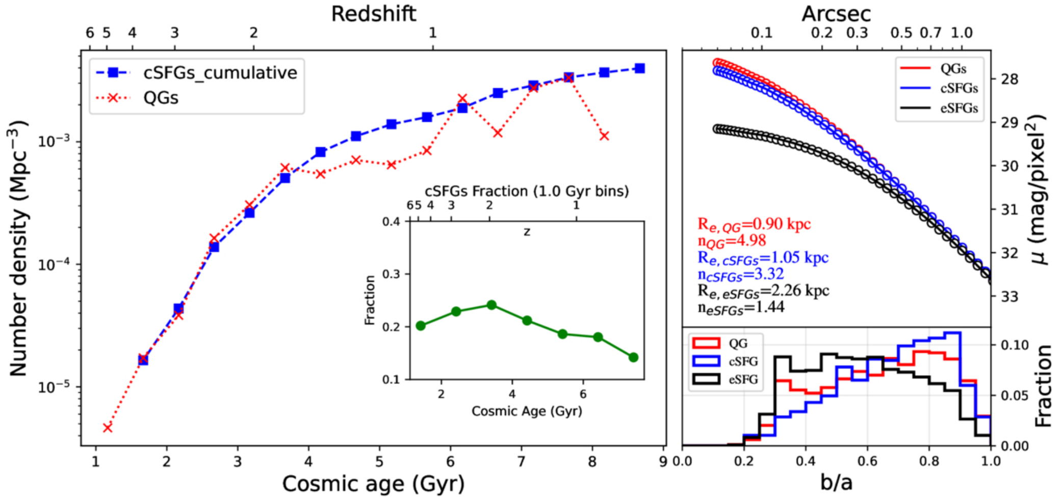
Figure 6. from Longyue Chen et al 2026 Astrophys. J. Lett. 1002 doi:10.3847/2041-8213/ae5a93 https://dx.doi.org/10.3847/2041-8213/ae5a93 © 2026. The Author(s). Published by the American Astronomical Society.
