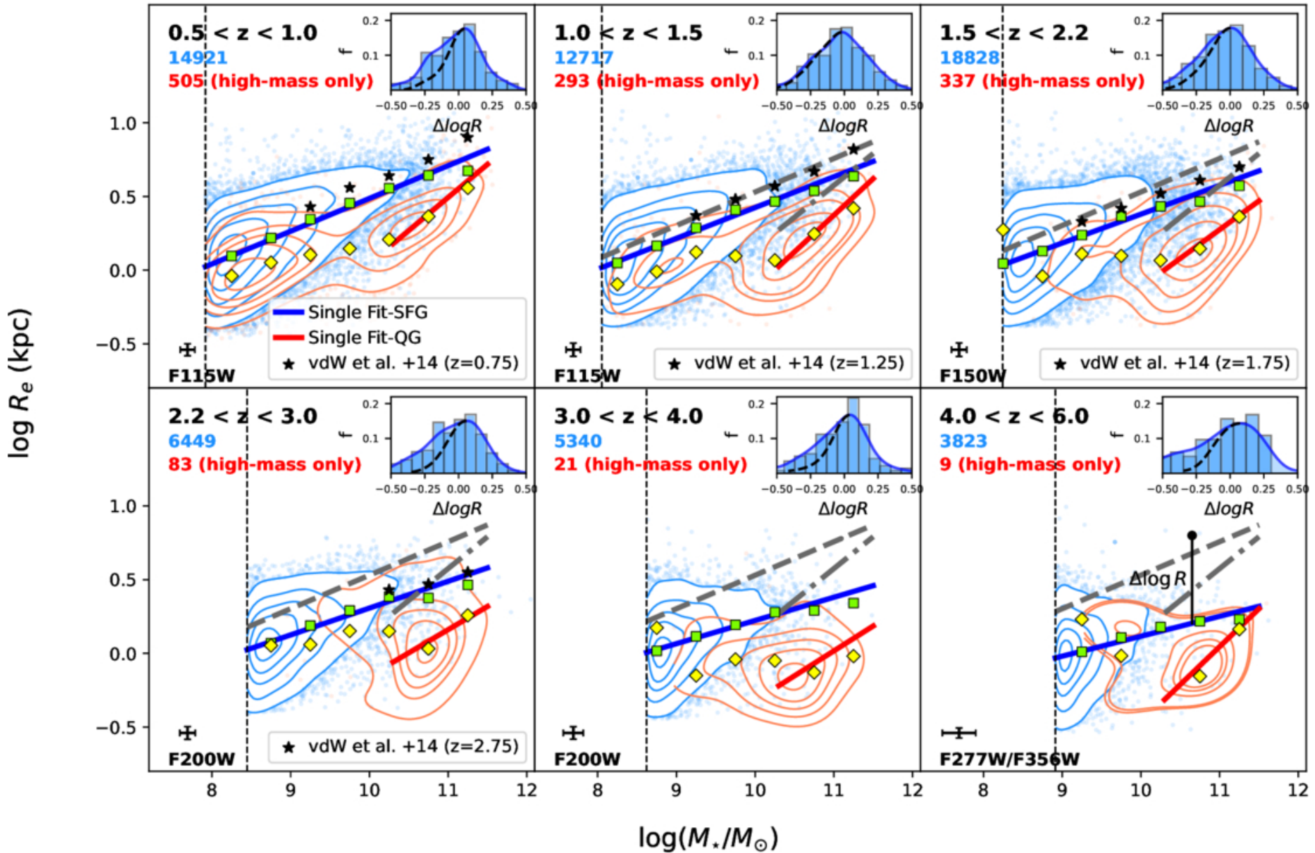
Figure 3. from Longyue Chen et al 2026 Astrophys. J. Lett. 1002 doi:10.3847/2041-8213/ae5a93 https://dx.doi.org/10.3847/2041-8213/ae5a93 © 2026. The Author(s). Published by the American Astronomical Society.
