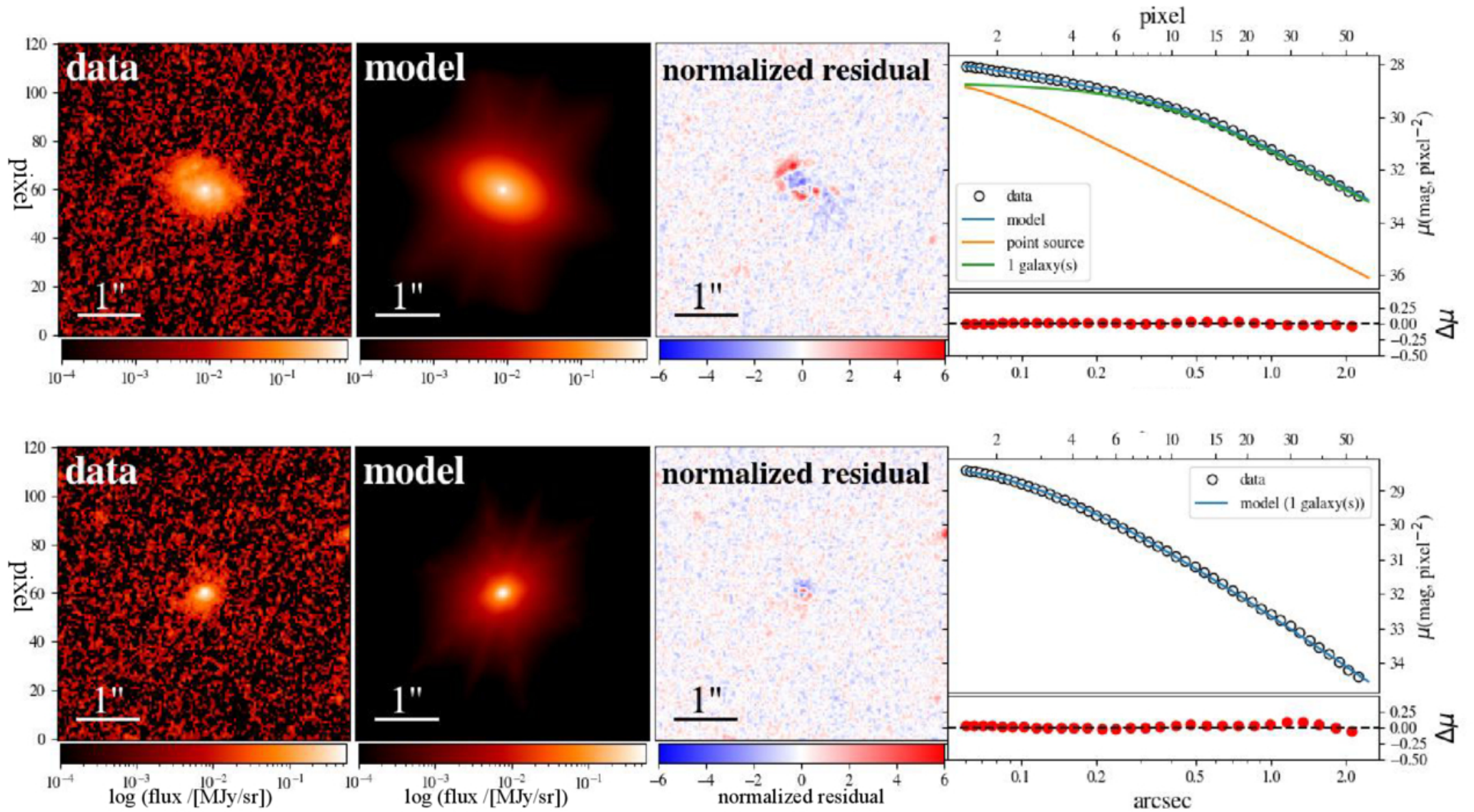
Figure 2. from Longyue Chen et al 2026 Astrophys. J. Lett. 1002 doi:10.3847/2041-8213/ae5a93 https://dx.doi.org/10.3847/2041-8213/ae5a93 © 2026. The Author(s). Published by the American Astronomical Society.
