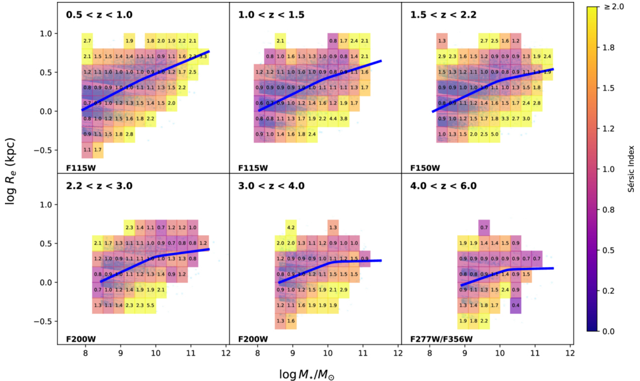
Figure E2. from Longyue Chen et al 2026 Astrophys. J. Lett. 1002 doi:10.3847/2041-8213/ae5a93 https://dx.doi.org/10.3847/2041-8213/ae5a93 © 2026. The Author(s). Published by the American Astronomical Society.
