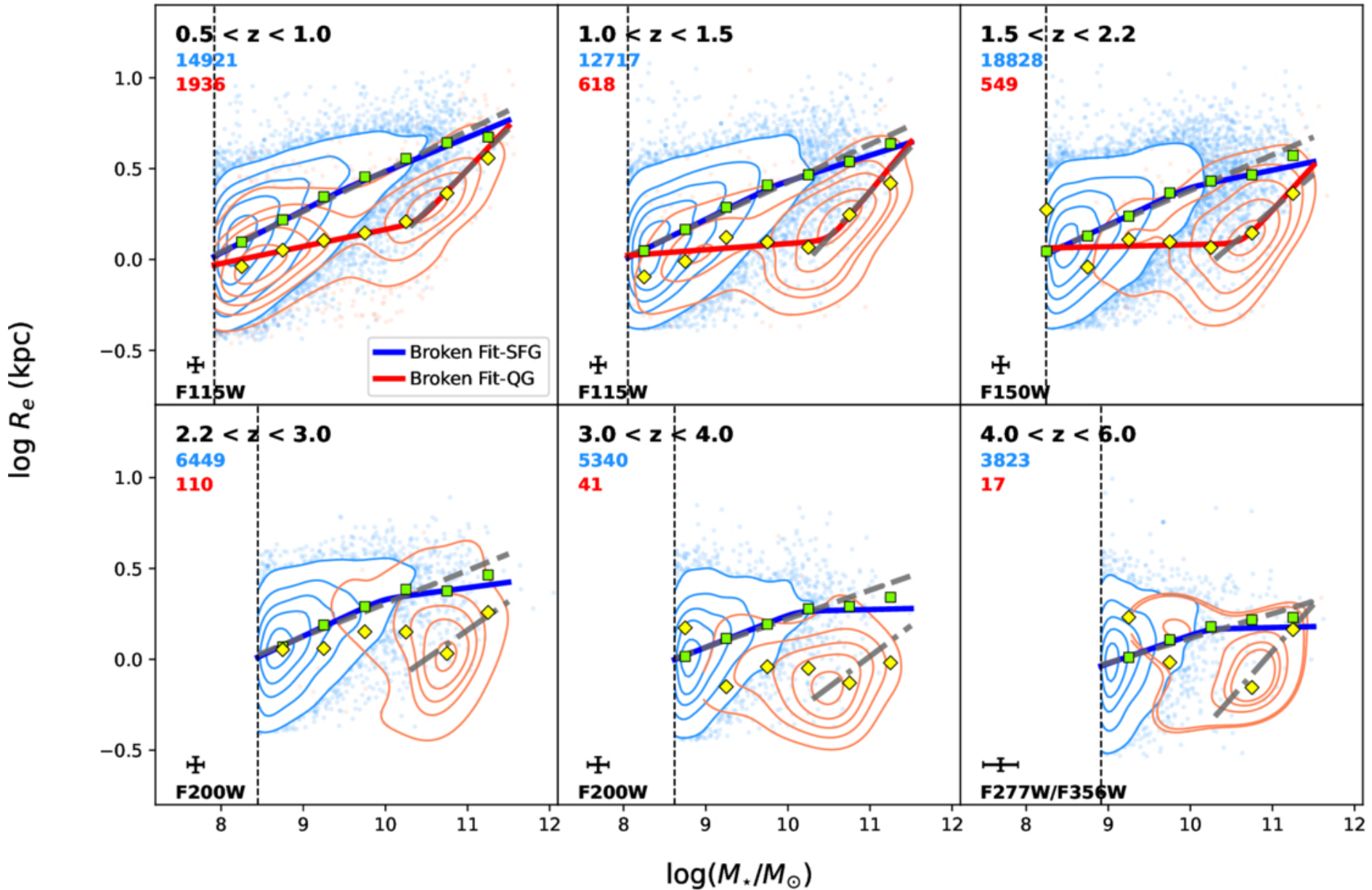
Figure E1. from Longyue Chen et al 2026 Astrophys. J. Lett. 1002 doi:10.3847/2041-8213/ae5a93 https://dx.doi.org/10.3847/2041-8213/ae5a93 © 2026. The Author(s). Published by the American Astronomical Society.
