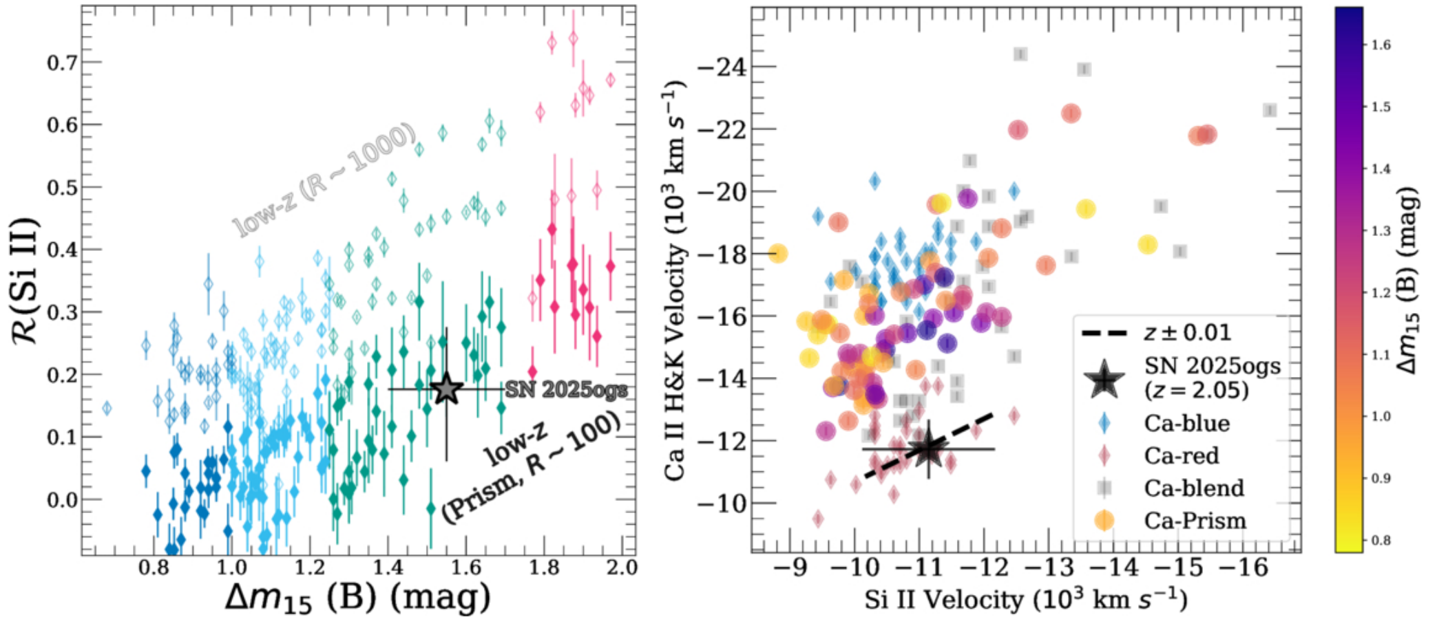
Figure 7. from M. R. Siebert et al 2026 Astrophys. J. Lett. 1002 doi:10.3847/2041-8213/ae5a37 https://dx.doi.org/10.3847/2041-8213/ae5a37 © 2026. The Author(s). Published by the American Astronomical Society.
