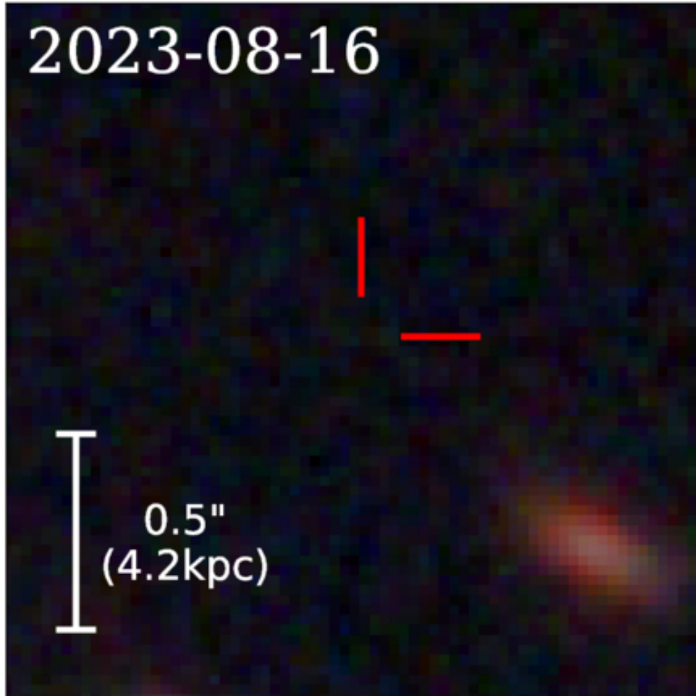
Figure 1. from M. R. Siebert et al 2026 Astrophys. J. Lett. 1002 doi:10.3847/2041-8213/ae5a37 https://dx.doi.org/10.3847/2041-8213/ae5a37 © 2026. The Author(s). Published by the American Astronomical Society.
