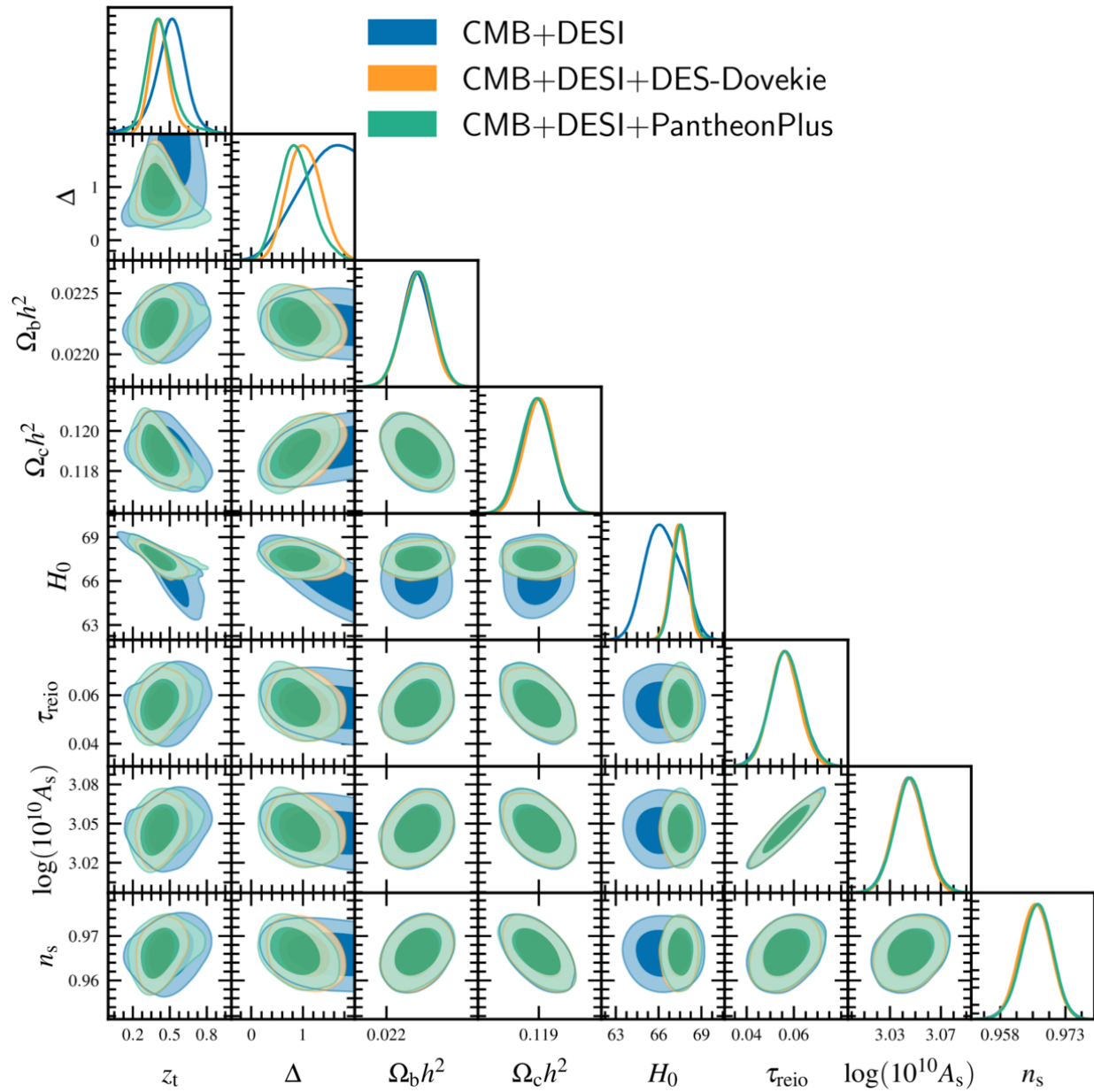
Figure 1. from Xiaolei Li et al 2026 Astrophys. J. Lett. 1001 doi:10.3847/2041-8213/ae5a36 https://dx.doi.org/10.3847/2041-8213/ae5a36 © 2026. The Author(s). Published by the American Astronomical Society.
