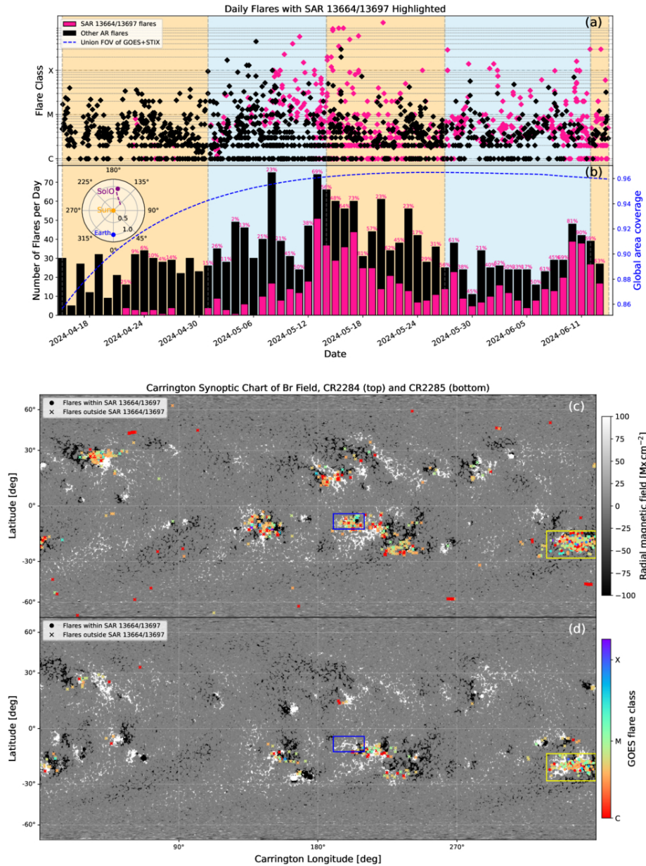
Figure 1. from Yue Zhang et al 2026 Astrophys. J. Lett. 1001 doi:10.3847/2041-8213/ae5a2f https://dx.doi.org/10.3847/2041-8213/ae5a2f © 2026. The Author(s). Published by the American Astronomical Society.
