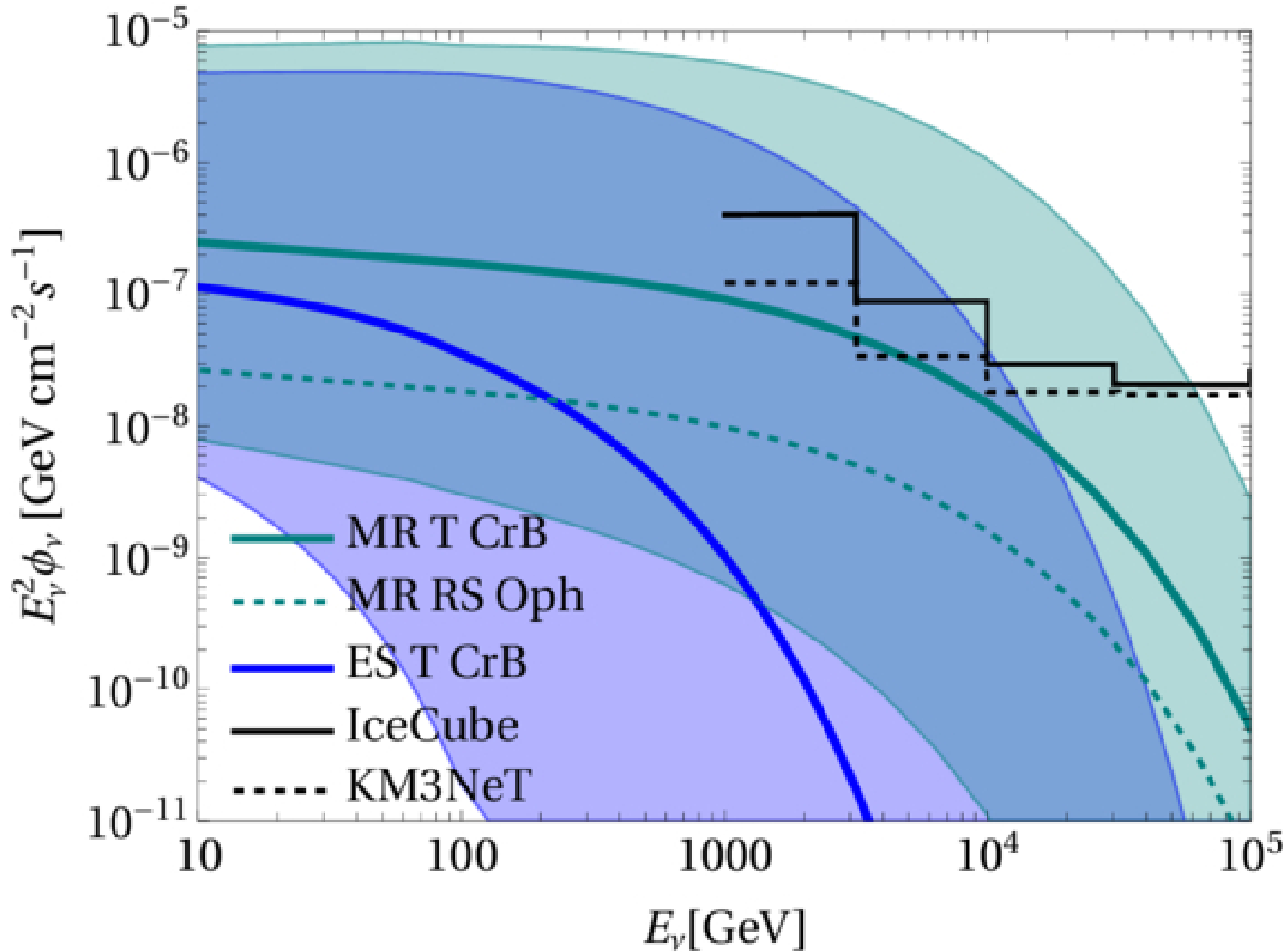
Figure 3. from Prantik Sarmah et al 2026 Astrophys. J. Lett. 1001 doi:10.3847/2041-8213/ae595a https://dx.doi.org/10.3847/2041-8213/ae595a © 2026. The Author(s). Published by the American Astronomical Society.
