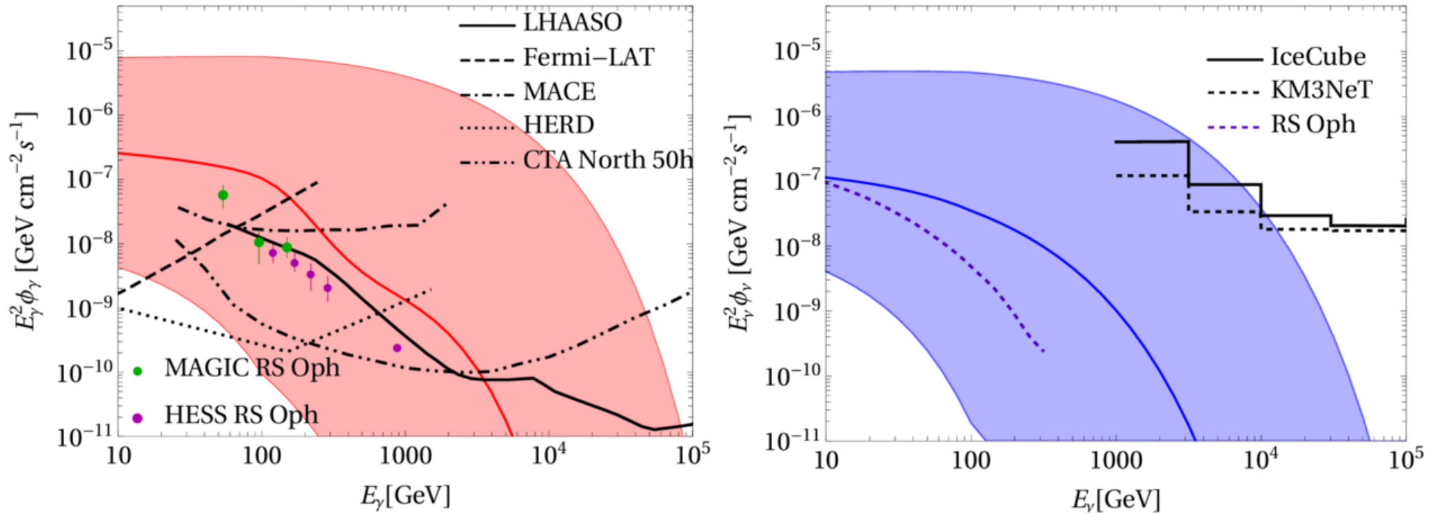
Figure 2. from Prantik Sarmah et al 2026 Astrophys. J. Lett. 1001 doi:10.3847/2041-8213/ae595a https://dx.doi.org/10.3847/2041-8213/ae595a © 2026. The Author(s). Published by the American Astronomical Society.
