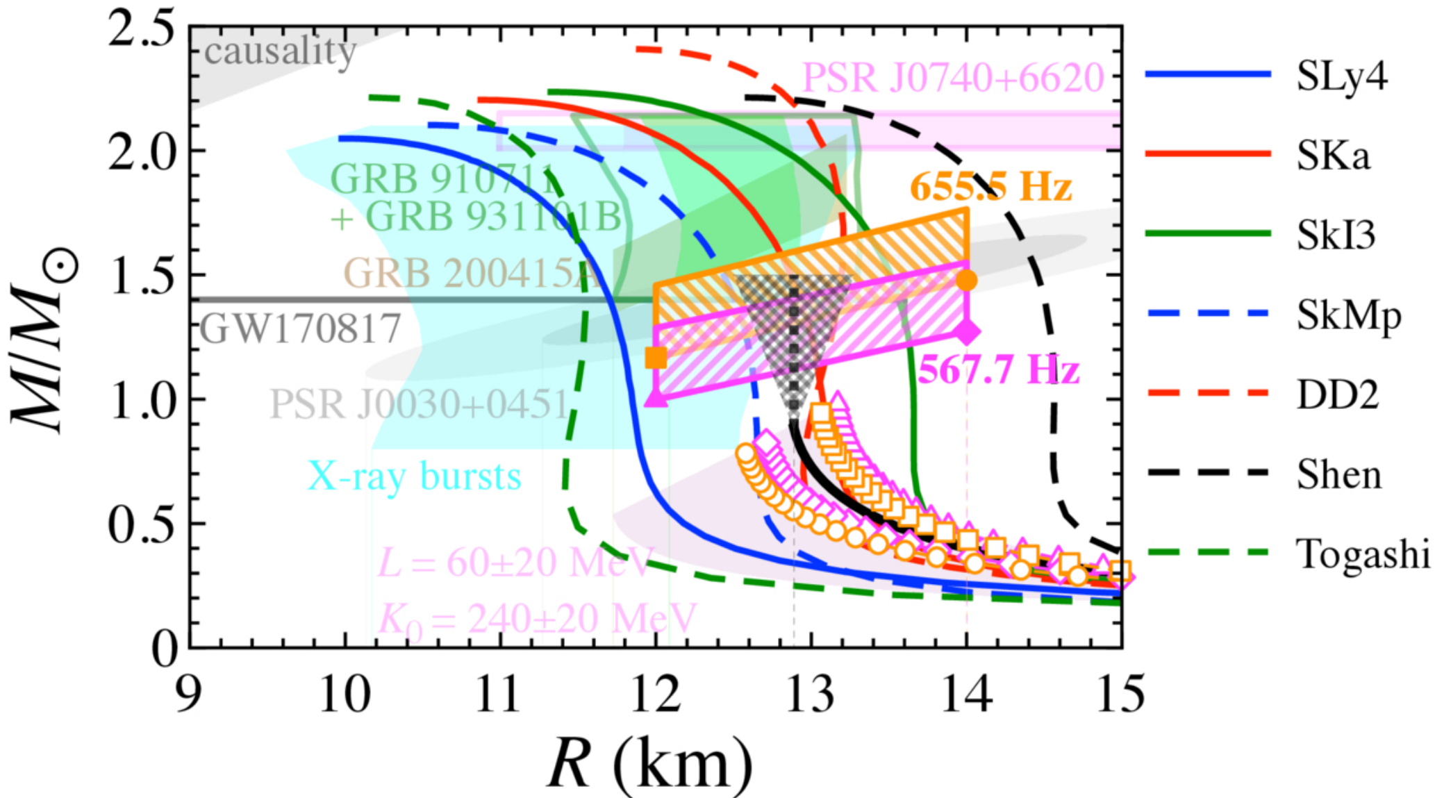
Figure 6. from Hajime Sotani et al 2026 Astrophys. J. Lett. 1001 doi:10.3847/2041-8213/ae5896 https://dx.doi.org/10.3847/2041-8213/ae5896 © 2026. The Author(s). Published by the American Astronomical Society.
