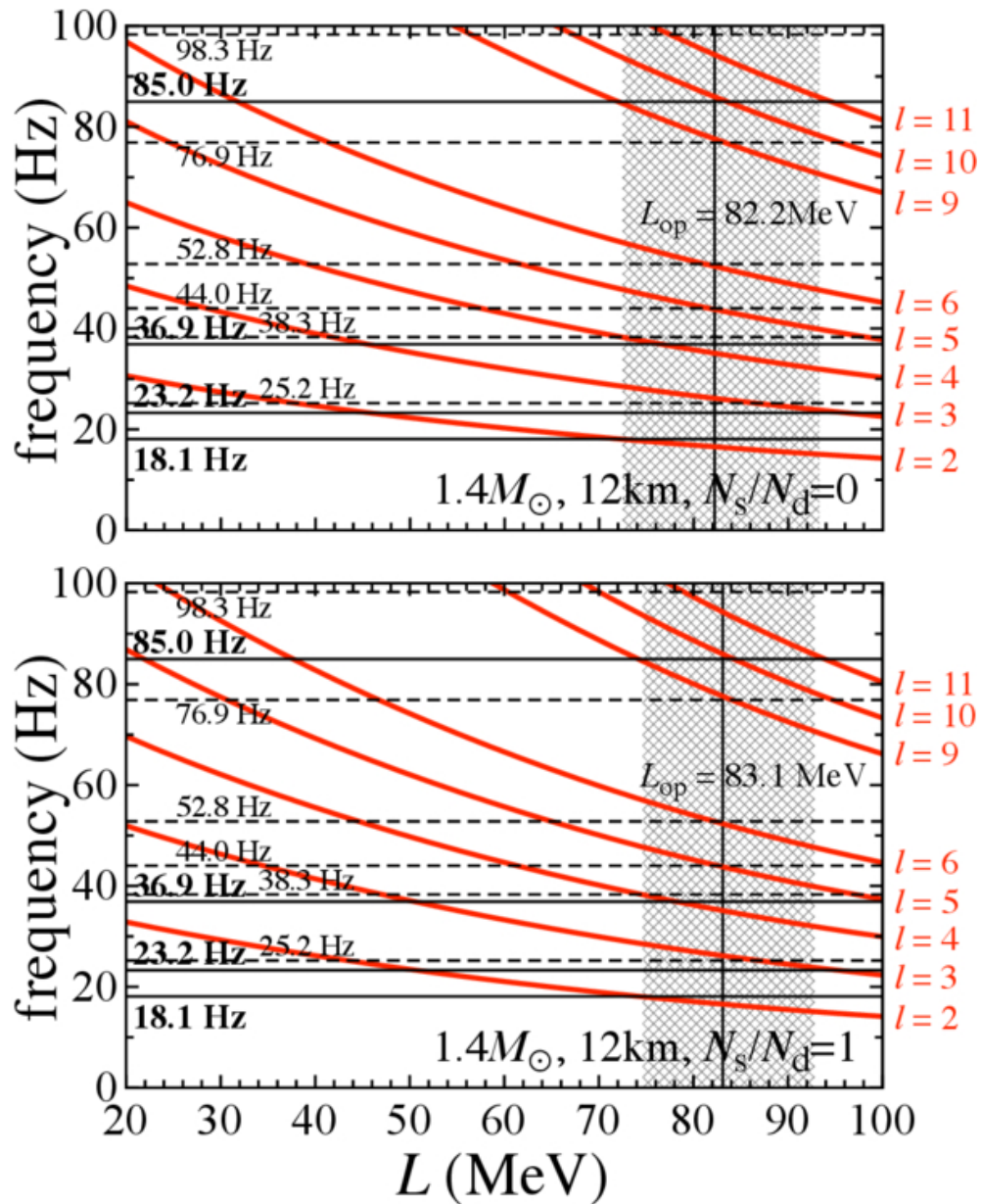
Figure 1. from Hajime Sotani et al 2026 Astrophys. J. Lett. 1001 doi:10.3847/2041-8213/ae5896 https://dx.doi.org/10.3847/2041-8213/ae5896 © 2026. The Author(s). Published by the American Astronomical Society.
