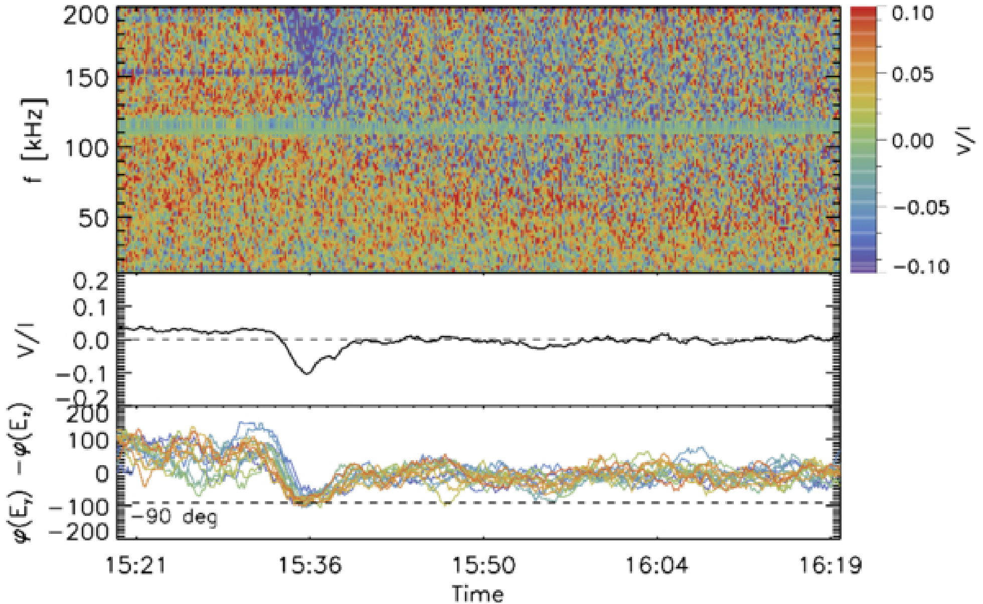
Figure 4. from Matthieu Kretzschmar et al 2026 Astrophys. J. Lett. 1001 doi:10.3847/2041-8213/ae5893 https://dx.doi.org/10.3847/2041-8213/ae5893 © 2026. The Author(s). Published by the American Astronomical Society.
