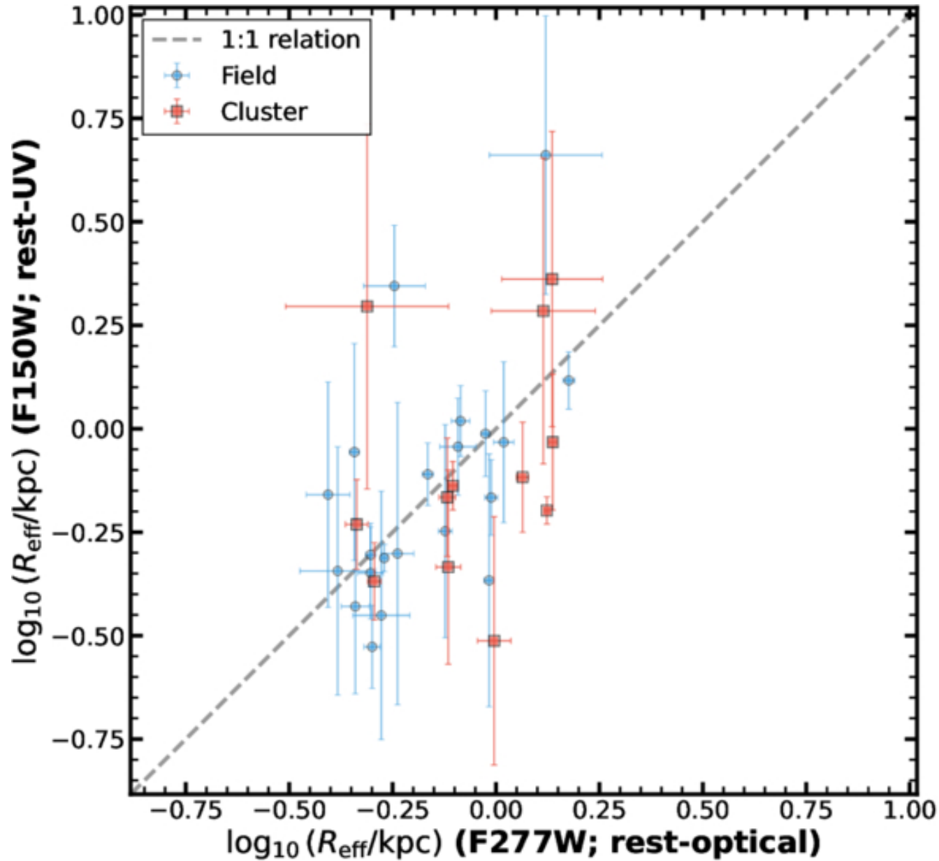
Figure 4. from Ronaldo Laishram et al 2026 Astrophys. J. Lett. 1002 doi:10.3847/2041-8213/ae5824 https://dx.doi.org/10.3847/2041-8213/ae5824 © 2026. The Author(s). Published by the American Astronomical Society.
