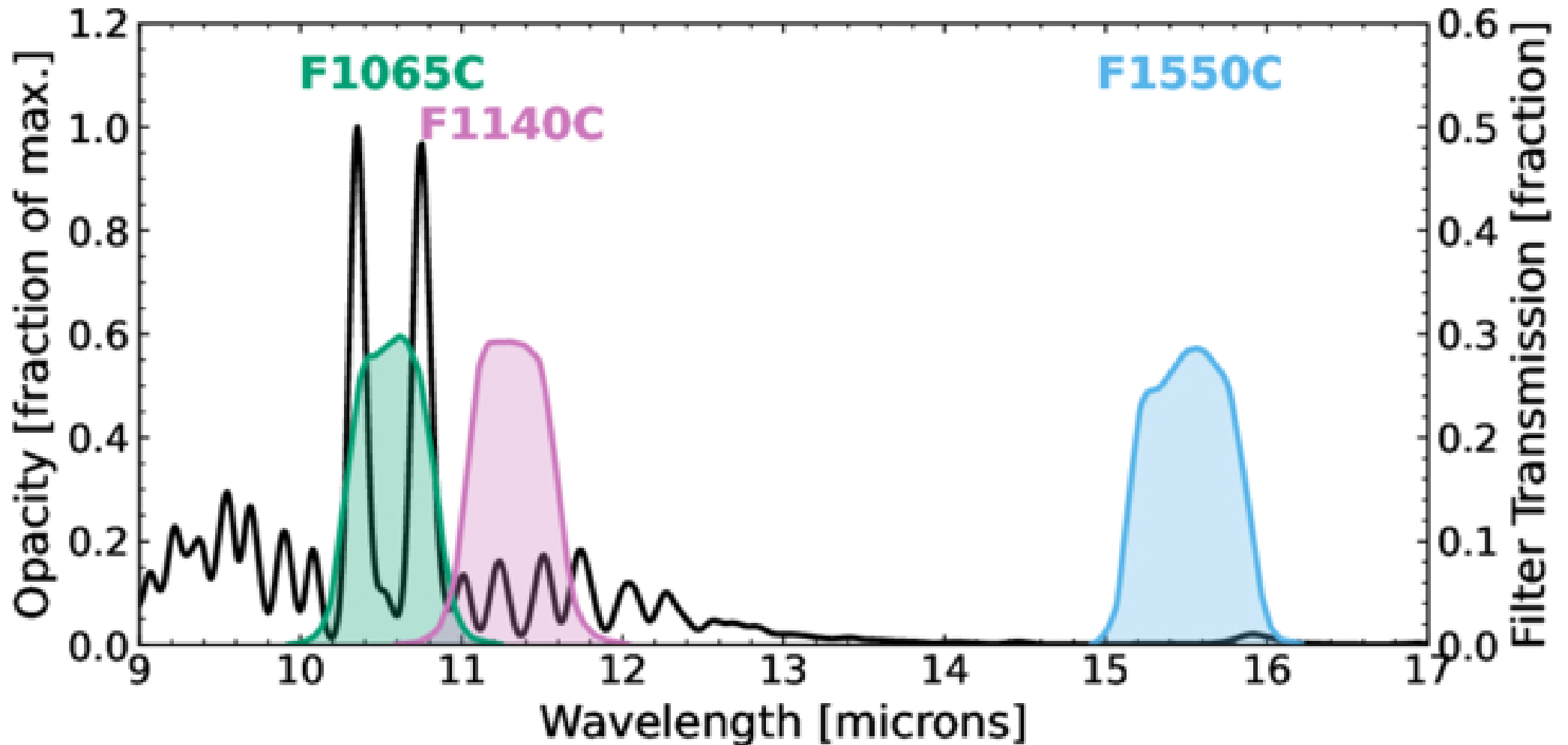
Figure 2. from Elisabeth C. Matthews et al 2026 Astrophys. J. Lett. 1002 doi:10.3847/2041-8213/ae5823 https://dx.doi.org/10.3847/2041-8213/ae5823 © 2026. The Author(s). Published by the American Astronomical Society.
