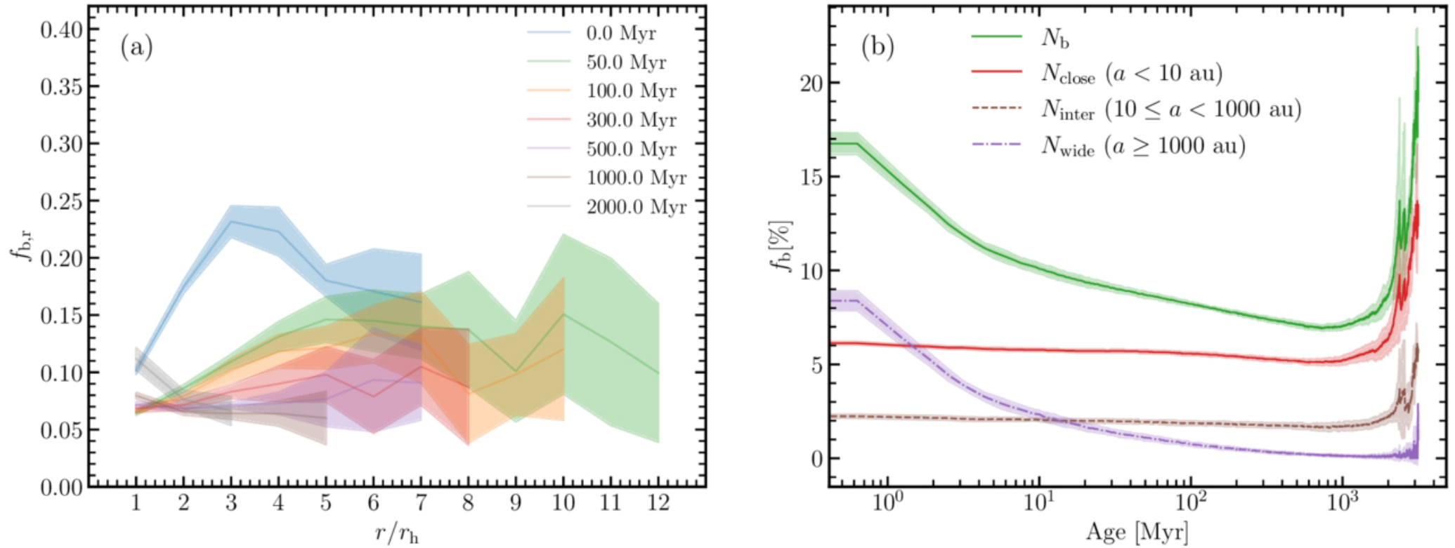
Figure 4. from Abylay Bissekenov et al 2026 Astrophys. J. Lett. 1001 doi:10.3847/2041-8213/ae5819 https://dx.doi.org/10.3847/2041-8213/ae5819 © 2026. The Author(s). Published by the American Astronomical Society.
