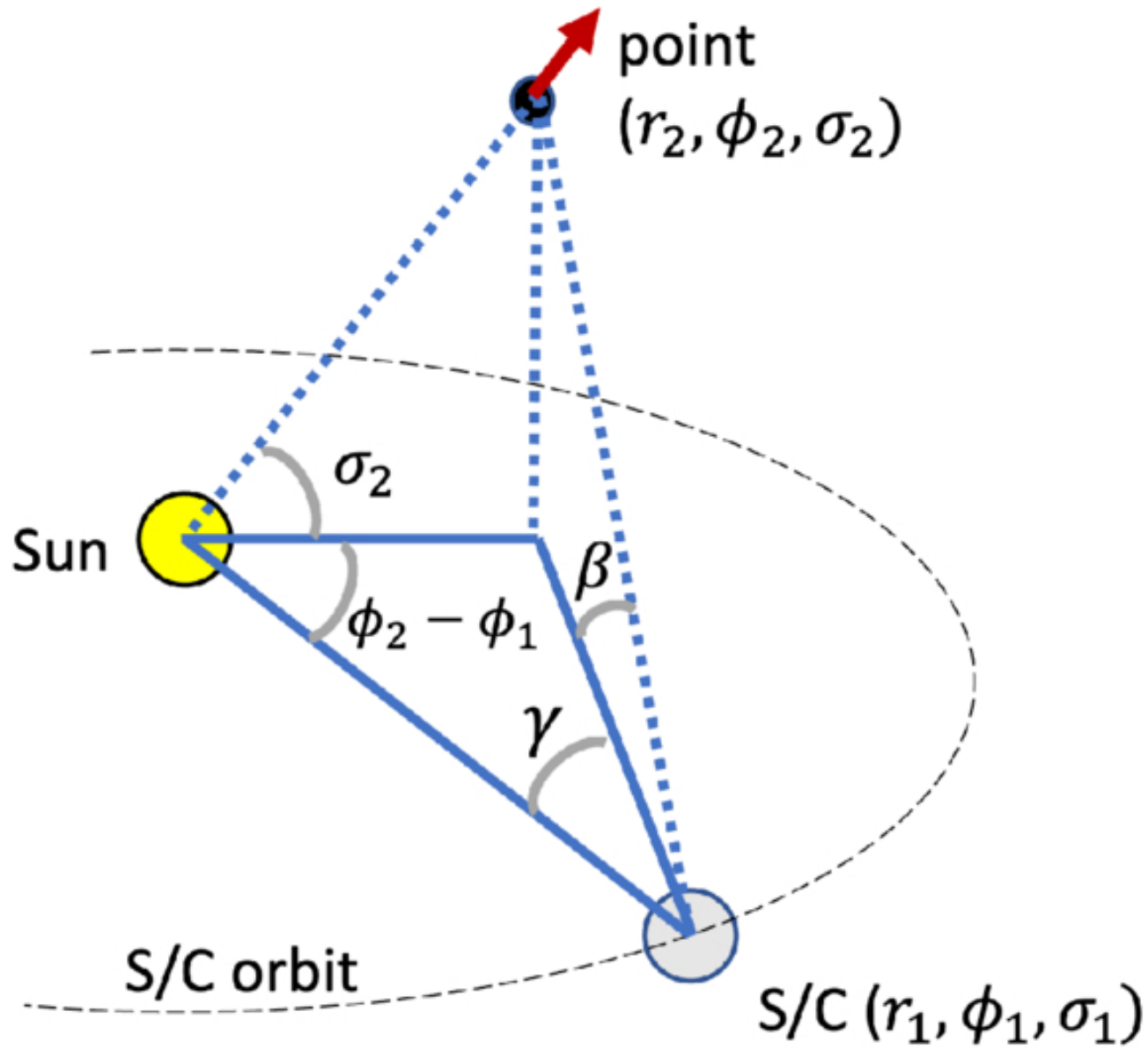
Figure 2. from Carlos R. Braga et al 2026 Astrophys. J. Lett. 1002 doi:10.3847/2041-8213/ae57a7 https://dx.doi.org/10.3847/2041-8213/ae57a7 © 2026. The Author(s). Published by the American Astronomical Society.
