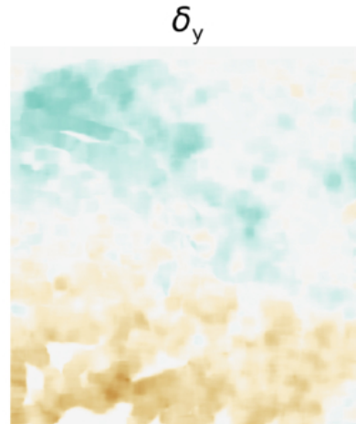
Figure 1. from Carlos R. Braga et al 2026 Astrophys. J. Lett. 1002 doi:10.3847/2041-8213/ae57a7 https://dx.doi.org/10.3847/2041-8213/ae57a7 © 2026. The Author(s). Published by the American Astronomical Society.
