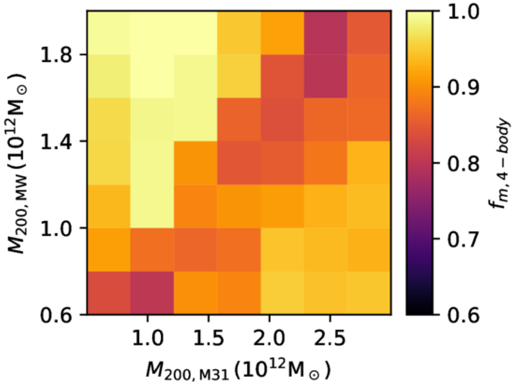
Figure E1. from Hao Wu et al 2026 Astrophys. J. Lett. 1001 doi:10.3847/2041-8213/ae5799 https://dx.doi.org/10.3847/2041-8213/ae5799 © 2026. The Author(s). Published by the American Astronomical Society.
