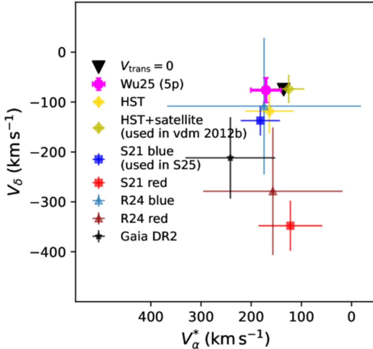
Figure 1. from Hao Wu et al 2026 Astrophys. J. Lett. 1001 doi:10.3847/2041-8213/ae5799 https://dx.doi.org/10.3847/2041-8213/ae5799 © 2026. The Author(s). Published by the American Astronomical Society.
