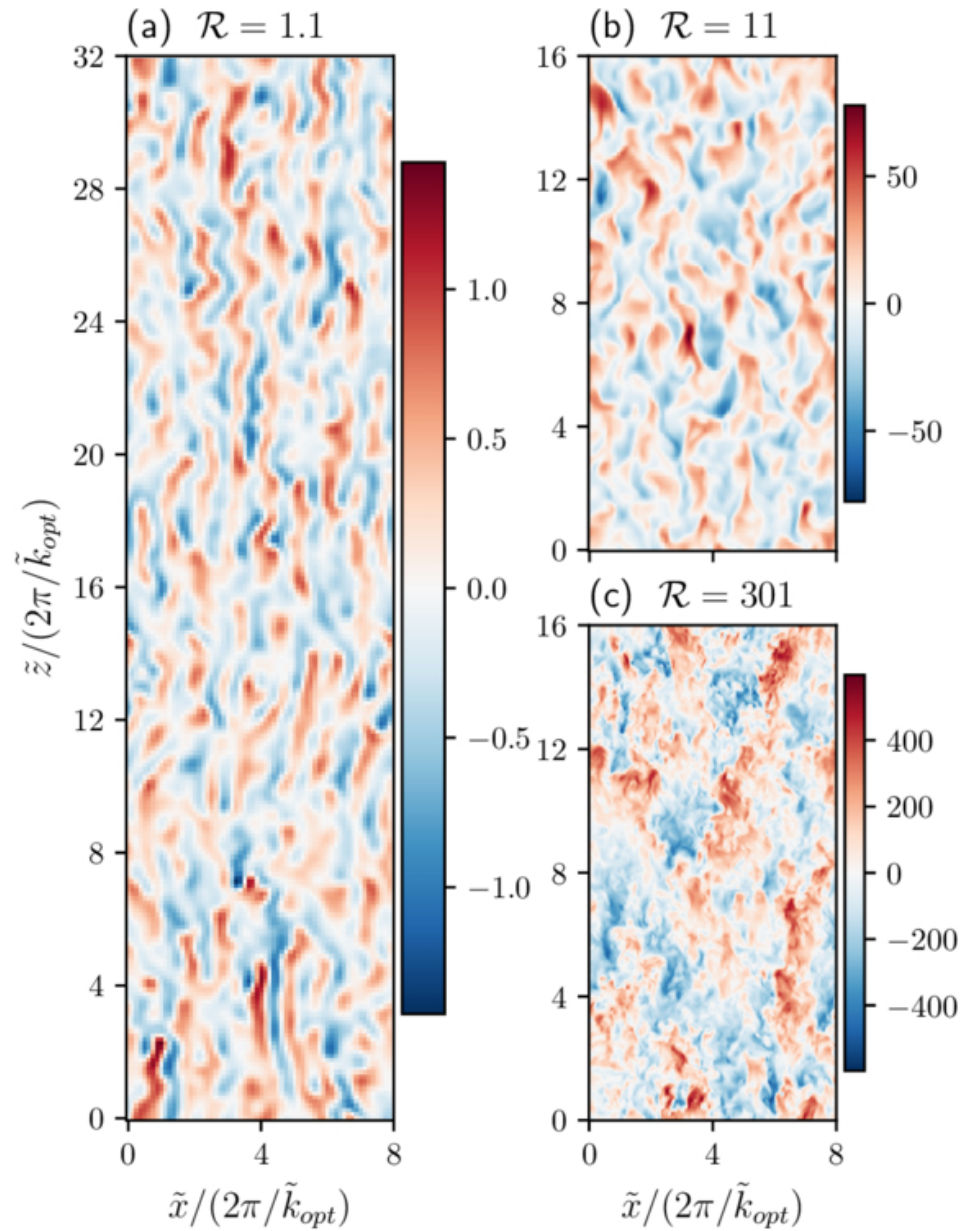
Figure 2. from Adrian E. Fraser 2026 Astrophys. J. Lett. 1001 doi:10.3847/2041-8213/ae5796 https://dx.doi.org/10.3847/2041-8213/ae5796 © 2026. The Author(s). Published by the American Astronomical Society.
